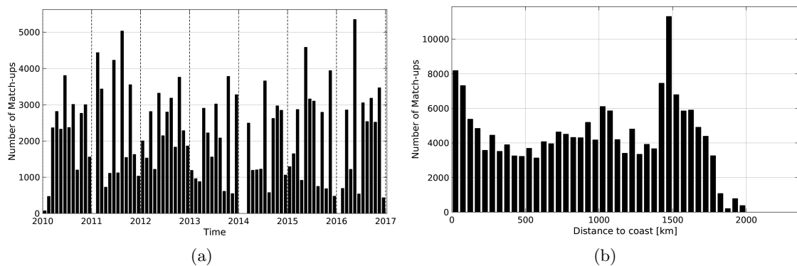
Figure 1: Number of match-ups between TSG-LEGOS-DM and SMOS-L3-CATDS-CPDC-V3-10DAYS-25KM SSS as a function of time (a) and as function of the distance to coast (b) over the Amazon and Orinoco river plumes Pi-MEP region and for the full satellite product period.
