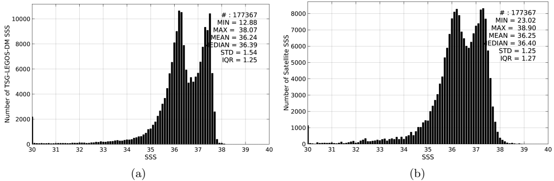
Figure 2: Histograms of SSS from TSG-LEGOS-DM (a) and SMOS-L3-CATDS-CPDC-V3-10DAYS-25KM (b) considering all match-up pairs per bins of 0.1 over the Amazon and Orinoco river plumes Pi-MEP region and for the full satellite product period.
