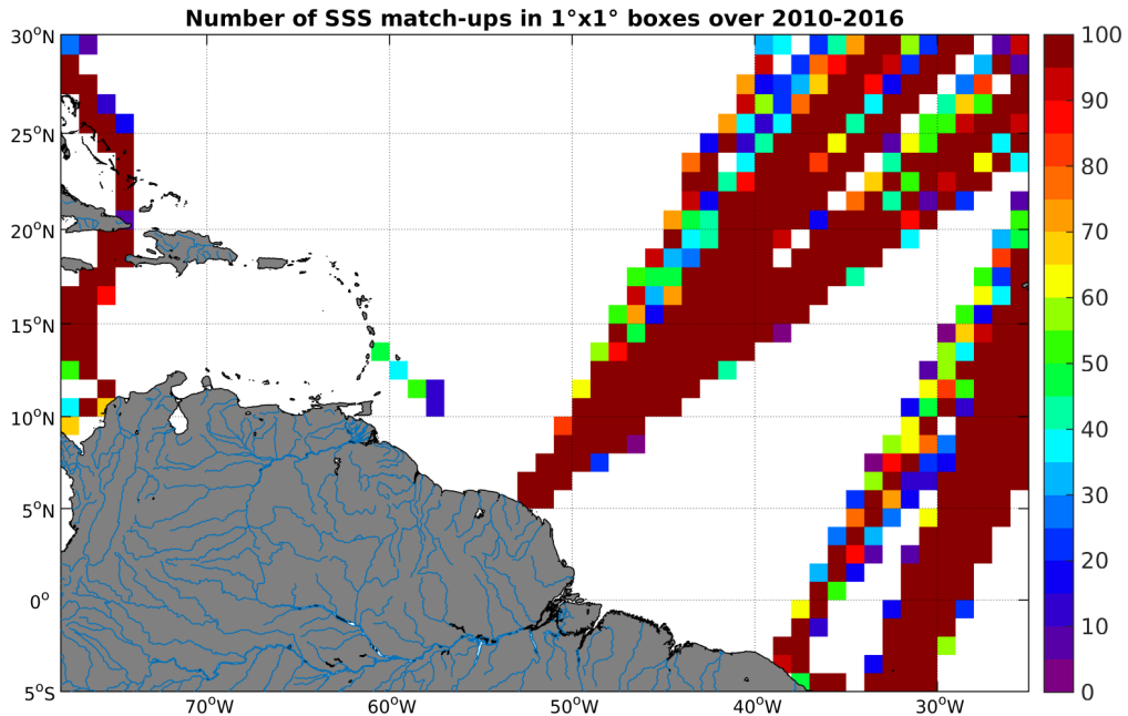
Figure 4: Number of SSS match-ups between TSG-LEGOS-DM SSS and the SMOS-L3-CATDS-CPDC-V3-10DAYS-25KM SSS product for the Amazon and Orinoco river plumes Pi-MEP region over 1^\circ \times 1^\circ boxes and for the full satellite product period.
