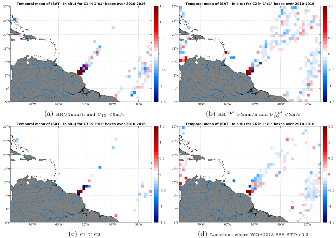
Figure 12: Temporal mean gridded over spatial boxes of size 1^\circ \times 1^\circ of \Delta SSS (SMOS-L3-CATDS-CPDC-V3-10DAYS-25KM - TSG-LEGOS-DM) for 4 different subdatasets corresponding to: RR > 1\text{mm/h} and U_{10} < 5\text{m/s} (a), RR^{10d} > 5\text{mm/h} and U_{10}^{10d} < 5\text{m/s} (b), C1 U C2 (c), Locations where WOA2013 SSS STD > 0.2 (d).
