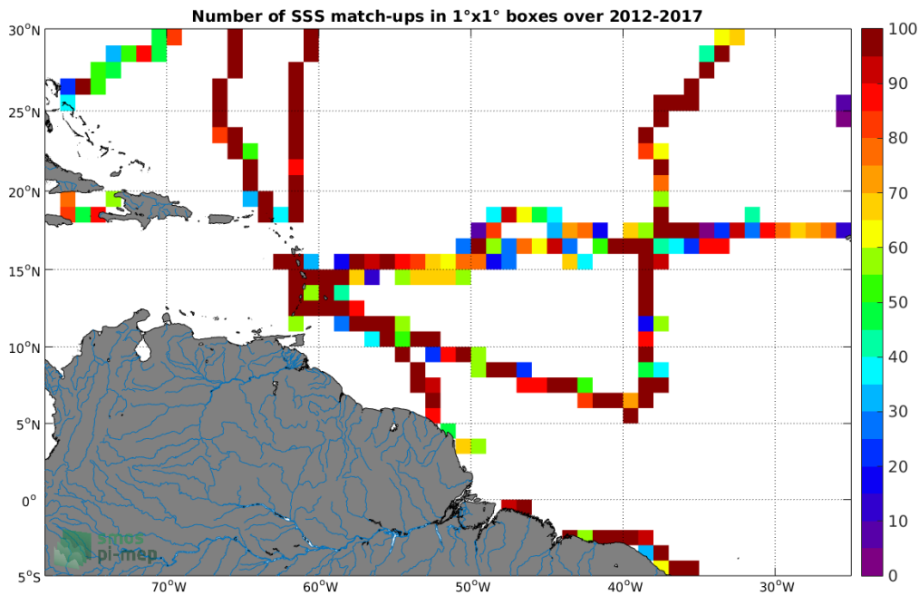
Figure 4: Number of SSS match-ups between TSG-GOSUD-Sailing-ship SSS and the SMOS-L3-CATDS-CPDC-V3-10DAYS-25KM SSS product for the Amazon and Orinoco river plumes Pi-MEP region over 1°x1° boxes and for the full satellite product period.
