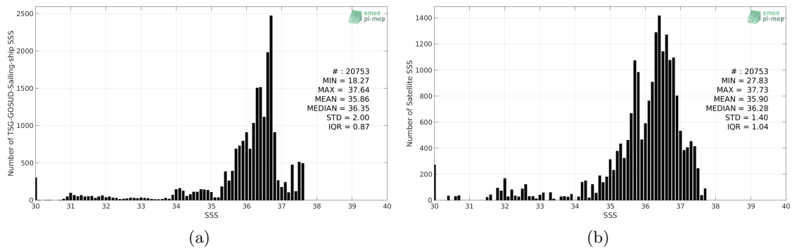
Figure 2: Histograms of SSS from TSG-GOSUD-Sailing-ship (a) and SMOS-L3-CATDS-CPDC-V3-10DAYS-25KM (b) considering all match-up pairs per bins of 0.1 over the Amazon and Orinoco river plumes Pi-MEP region and for the full satellite product period.
