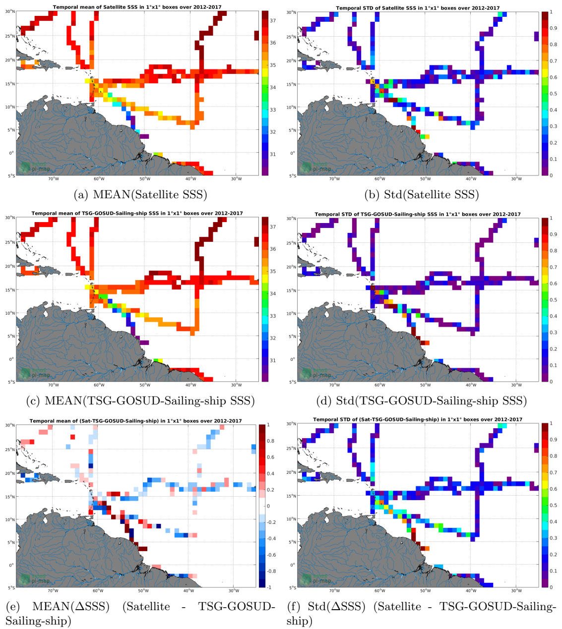
Figure 6: Temporal mean (left) and Std (right) of SSS from SMOS-L3-CATDS-CPDC-V3-10DAYS-25KM (top), TSG-GOSUD-Sailing-ship (middle), and of \Delta SSS (Satellite - TSG-GOSUD-Sailing-ship). Only match-up pairs are used to generate these maps.
