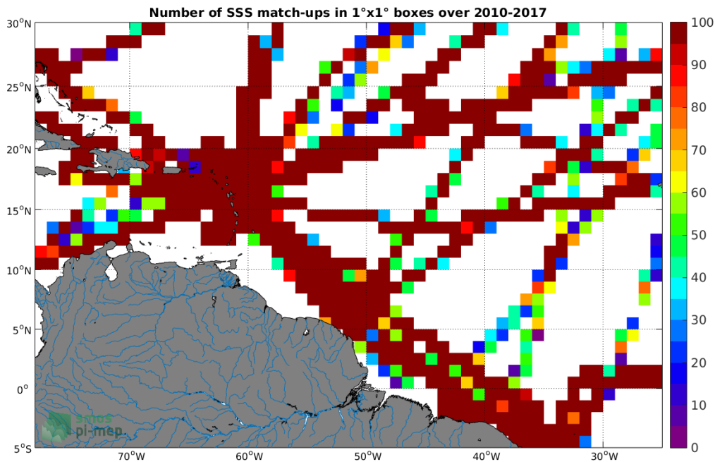
Figure 4: Number of SSS match-ups between TSG-GOSUD-Research-vessel SSS and the SMOS-L3-CATDS-CPDC-V3-10DAYS-25KM SSS product for the Amazon and Orinoco river plumes Pi-MEP region over 1°x1° boxes and for the full satellite product period.
