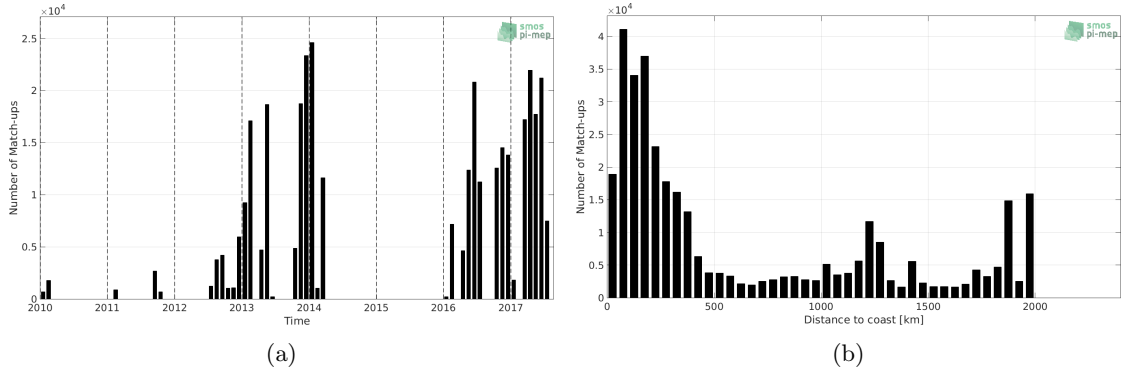
Figure 1: Number of match-ups between TSG-GOSUD-Research-vessel and SMOS-L3-CATDS-CPDC-V3-10DAYS-25KM SSS as a function of time (a) and as function of the distance to coast (b) over the Amazon and Orinoco river plumes Pi-MEP region and for the full satellite product period.
