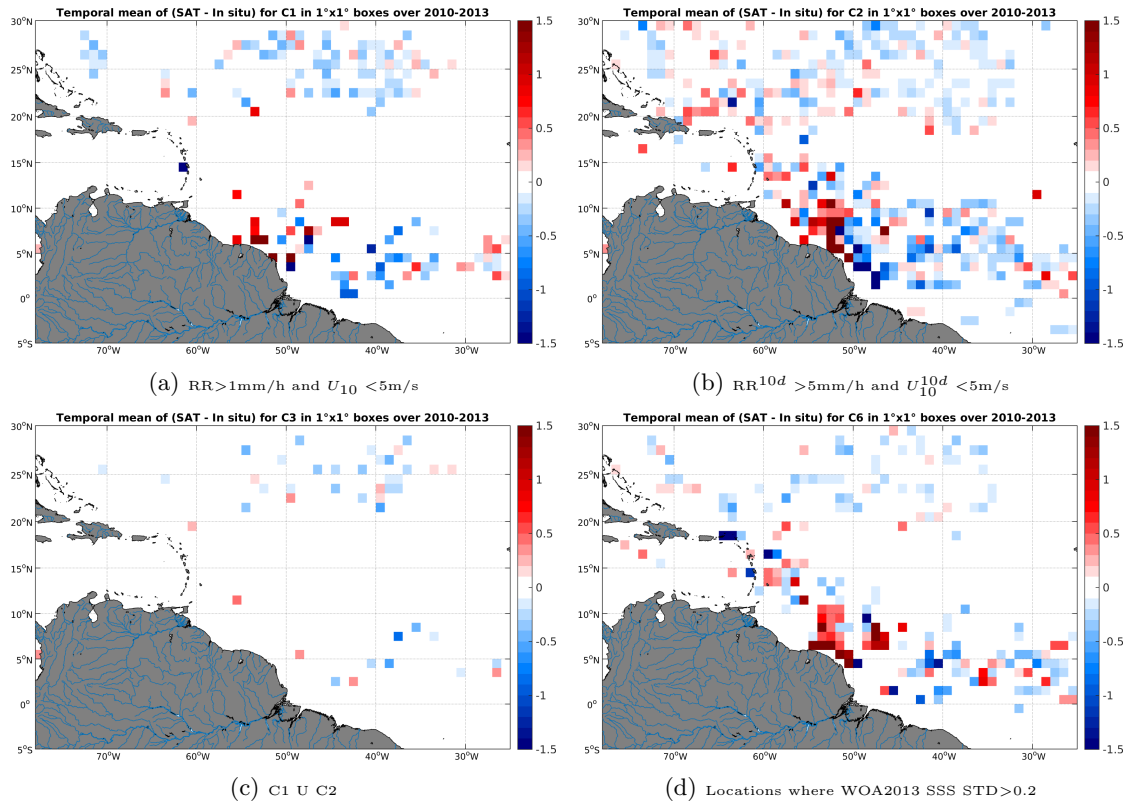
Figure 11: Temporal mean gridded over spatial boxes of size 1^\circ \times 1^\circ of \Delta SSS (SMOS-L3-CATDS-CPDC-V3-10DAYS-25KM - Surface drifters) for 4 different subdatasets corresponding to:RR >1 mm/h and U_{10} < 5 m/s (a), RR 10d > 5 mm/h and U_{10}^{10d} < 5 m/s (b), C1 U C2 (c),Locations where WOA2013 SSS STD > 0.2 (d).
