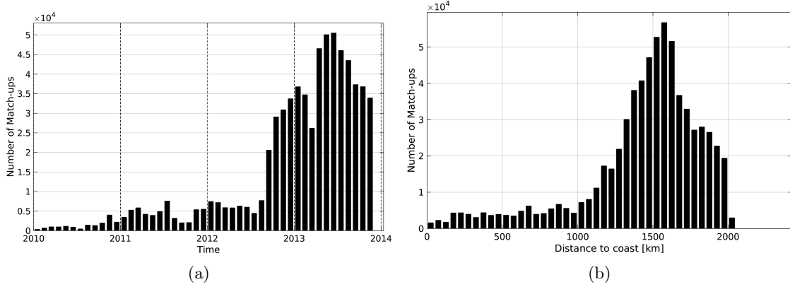
Figure 1: Number of match-ups between Surface drifters and SMOS-L3-CATDS-CPDC-V3-10DAYS-25KM SSS as a function of time (a) and as function of the distance to coast (b) over the Amazon and Orinoco river plumes Pi-MEP region and for the full satellite product period.
