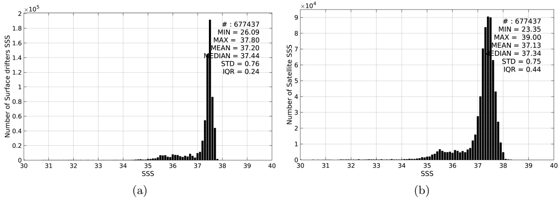
Figure 2: Histograms of SSS from Surface drifters (a) and SMOS-L3-CATDS-CPDC-V3-10DAYS-25KM (b) considering all match-up pairs per bins of 0.1 over the Amazon and Orinoco river plumes Pi-MEP region and for the full satellite product period.
