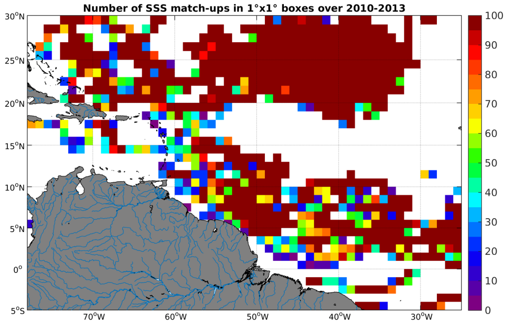
Figure 3: Number of SSS match-ups between Surface drifters SSS and the SMOS-L3-CATDS-CPDC-V3-10DAYS-25KM SSS product for the Amazon and Orinoco river plumes Pi-MEP region over 1°x1° boxes and for the full satellite product period.
