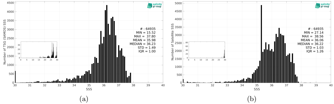
Figure 3: Histograms of SSS from TSG (SAMOS) (a) and SMOS SSS L3 v2 - 9-Days (BEC) (b) considering all match-up pairs per bins of 0.1 over the Amazon and Orinoco river plumes Pi-MEP region and for the full satellite product period.
