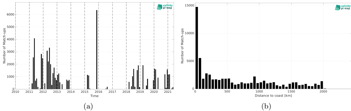
Figure 2: Number of match-ups between TSG (SAMOS) and SMOS SSS L3 v2 - 9-Days (BEC) SSS as a function of time (a) and as function of the distance to coast (b) over the Amazon and Orinoco river plumes Pi-MEP region and for the full satellite product period.
