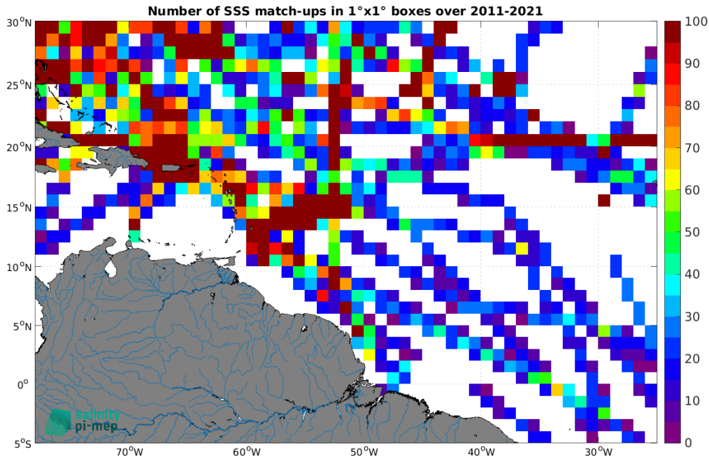
Figure 5: Number of SSS match-ups between TSG (SAMOS) SSS and the SMOS SSS L3 v2 - 9-Days (BEC) SSS product for the Amazon and Orinoco river plumes Pi-MEP region over 1^{\circ} \times 1^{\circ} boxes and for the full satellite product period.
