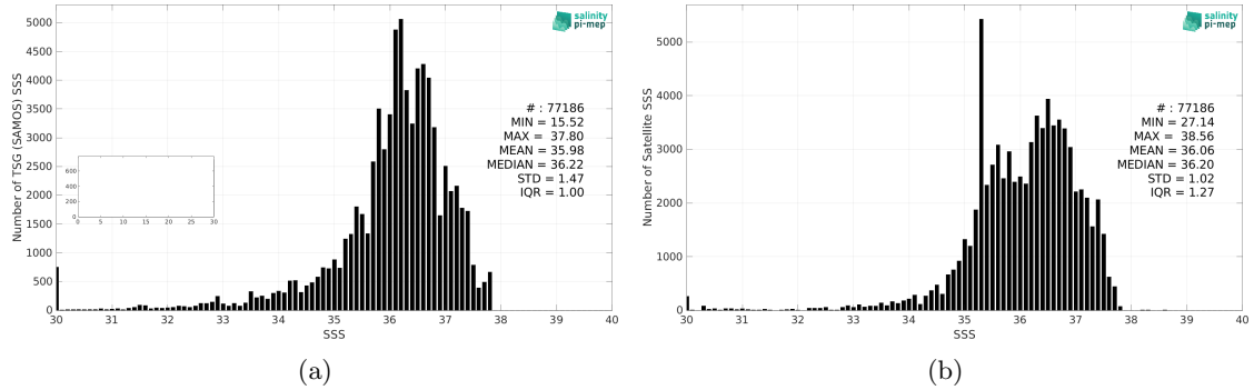
Figure 2: Histograms of SSS from TSG (SAMOS) (a) and SMOS SSS L3 v2 - 9-Days (BEC) (b) considering all match-up pairs per bins of 0.1 over the Amazon and Orinoco river plumes Pi-MEP region and for the full satellite product period.
