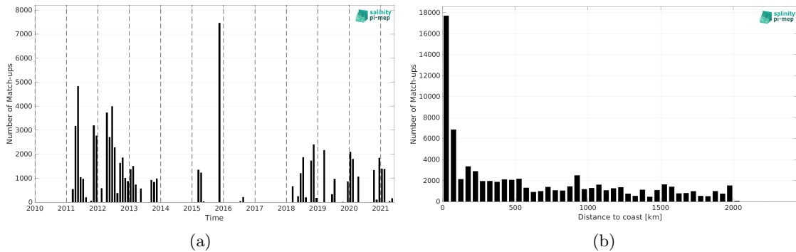
Figure 1: Number of match-ups between TSG (SAMOS) and SMOS SSS L3 v2 - 9-Days (BEC) SSS as a function of time (a) and as function of the distance to coast (b) over the Amazon and Orinoco river plumes Pi-MEP region and for the full satellite product period.
