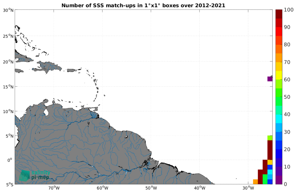
Figure 5: Number of SSS match-ups between TSG (Polarstern) SSS and the SMOS SSS L3 v2 - 9-Days (BEC) SSS product for the Amazon and Orinoco river plumes Pi-MEP region over 1^\circ \times 1^\circ boxes and for the full satellite product period.
