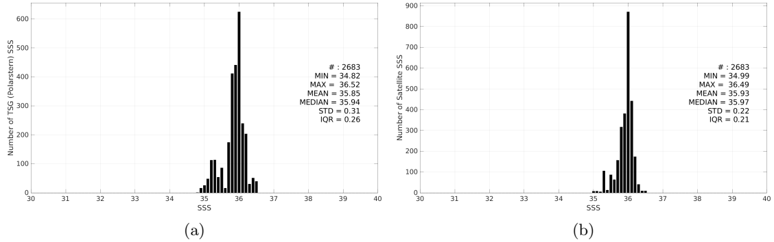
Figure 3: Histograms of SSS from TSG (Polarstern) (a) and SMOS SSS L3 v2 - 9-Days (BEC) (b) considering all match-up pairs per bins of 0.1 over the Amazon and Orinoco river plumes Pi-MEP region and for the full satellite product period.
