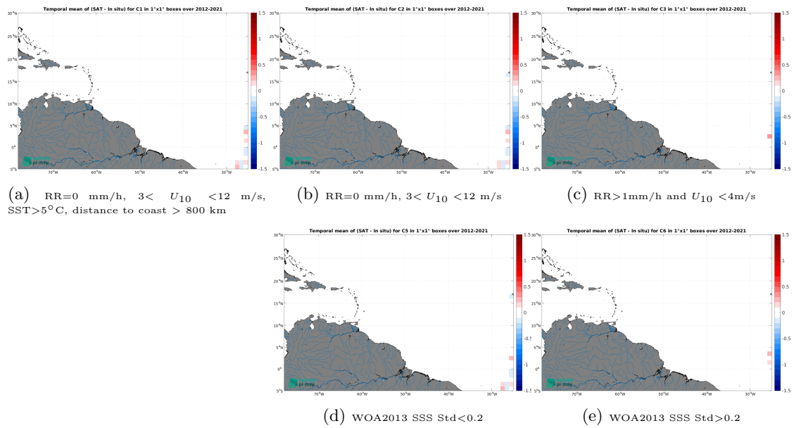
Figure 14: Temporal mean gridded over spatial boxes of size 1^\circ \times 1^\circ of \Delta SSS (SMOS SSS L3 v2 - 9-Days (BEC) - TSG (Polarstern)) for 5 different subdatasets corresponding to:RR=0 mm/h, 3 < U_{10} < 12 m/s, SST>5°C, distance to coast > 800 km (a), RR=0 mm/h, 3 < U_{10} < 12 m/s (b), RR>1mm/h and U_{10} < 4 m/s (c), WOA2013 SSS Std<0.2 (d), WOA2013 SSS Std>0.2 (e).
