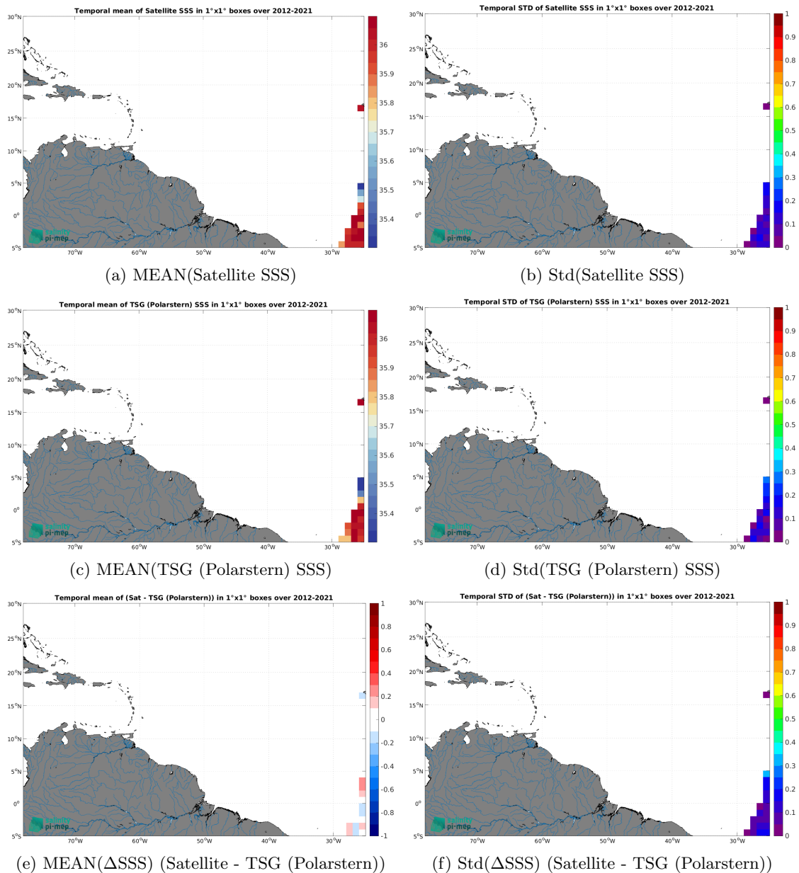
Figure 7: Temporal mean (left) and Std (right) of SSS from SMOS SSS L3 v2 - 9-Days (BEC) (top), TSG (Polarstern) (middle), and of \Delta SSS (Satellite - TSG (Polarstern)). Only match-up pairs are used to generate these maps.
