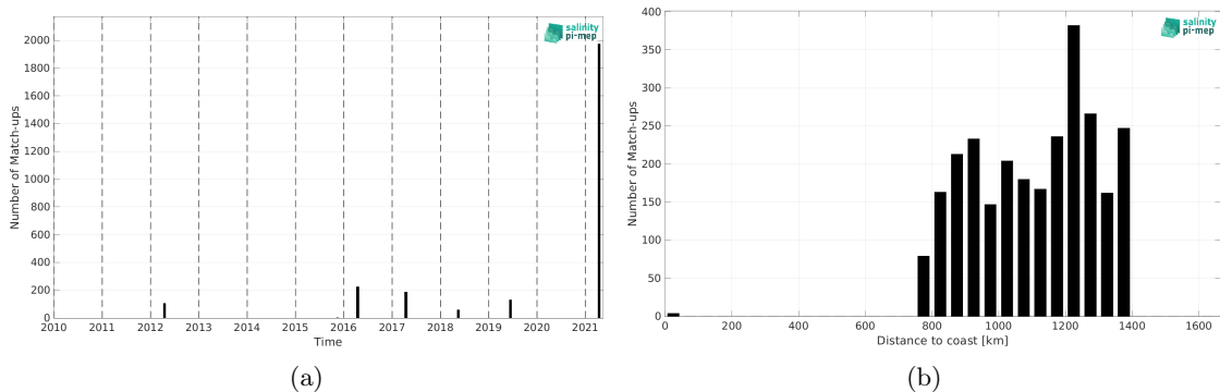
Figure 2: Number of match-ups between TSG (Polarstern) and SMOS SSS L3 v2 - 9-Days (BEC) SSS as a function of time (a) and as function of the distance to coast (b) over the Amazon and Orinoco river plumes Pi-MEP region and for the full satellite product period.
