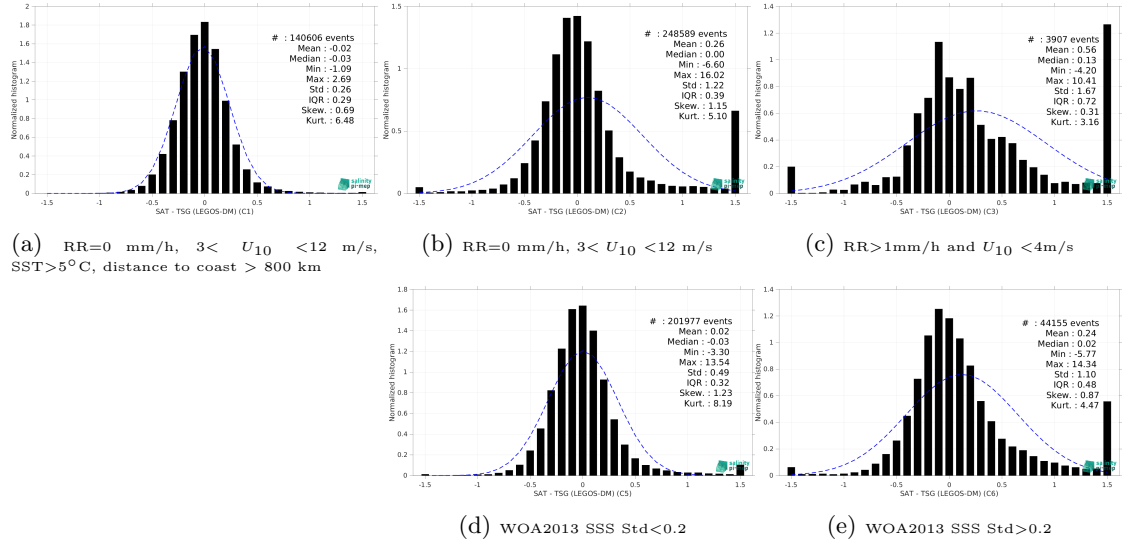
Figure 13: Normalized histogram of \Delta\text{SSS} (SMOS SSS L3 v2 - 9-Days (BEC) - TSG (LEGOS-DM)) for 5 different subdatasets corresponding to: RR=0 mm/h, 3 < U_{10} < 12 m/s, SST>5°C, distance to coast > 800 km (a), RR=0 mm/h, 3 < U_{10} < 12 m/s (b), RR>1mm/h and U_{10} < 4 m/s (c), WOA2013 SSS Std<0.2 (d), WOA2013 SSS Std>0.2 (e).
