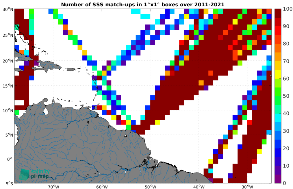
Figure 4: Number of SSS match-ups between TSG (LEGOS-DM) SSS and the SMOS SSS L3 v2 - 9-Days (BEC) SSS product for the Amazon and Orinoco river plumes Pi-MEP region over 1^{\circ} \times 1^{\circ} boxes and for the full satellite product period.
