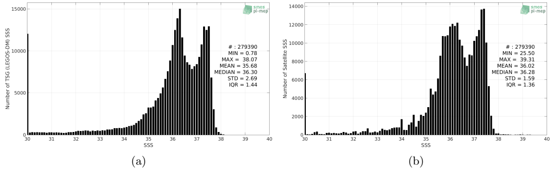
Figure 2: Histograms of SSS from TSG (LEGOS-DM) (a) and SMOS SSS L3 v2 - 9-Days (BEC) (b) considering all match-up pairs per bins of 0.1 over the Amazon and Orinoco river plumes Pi-MEP region and for the full satellite product period.
