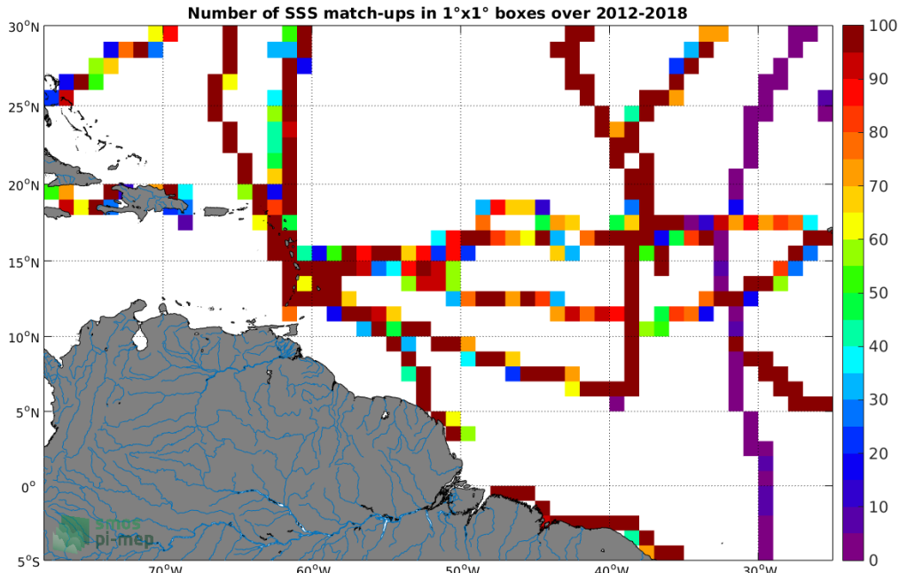
Figure 4: Number of SSS match-ups between TSG (GOSUD-Sailing-ship) SSS and the SMOS SSS L3 v2 - 9-Days (BEC) SSS product for the Amazon and Orinoco river plumes Pi-MEP region over 1^\circ \times 1^\circ boxes and for the full satellite product period.
