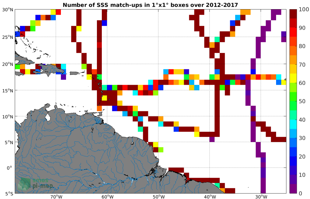
Figure 4: Number of SSS match-ups between TSG (GOSUD-Sailing-ship) SSS and the SMOS SSS L3 v2 - 9-Days (BEC) SSS product for the Amazon and Orinoco river plumes Pi-MEP region over 1°x1° boxes and for the full satellite product period.
