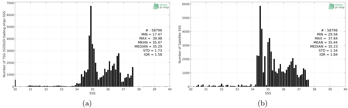
Figure 2: Histograms of SSS from TSG (GOSUD-Sailing-ship) (a) and SMOS L3 v2 - 9-Days (BEC) (b) considering all match-up pairs per bins of 0.1 over the Amazon and Orinoco river plumes Pi-MEP region and for the full satellite product period.
