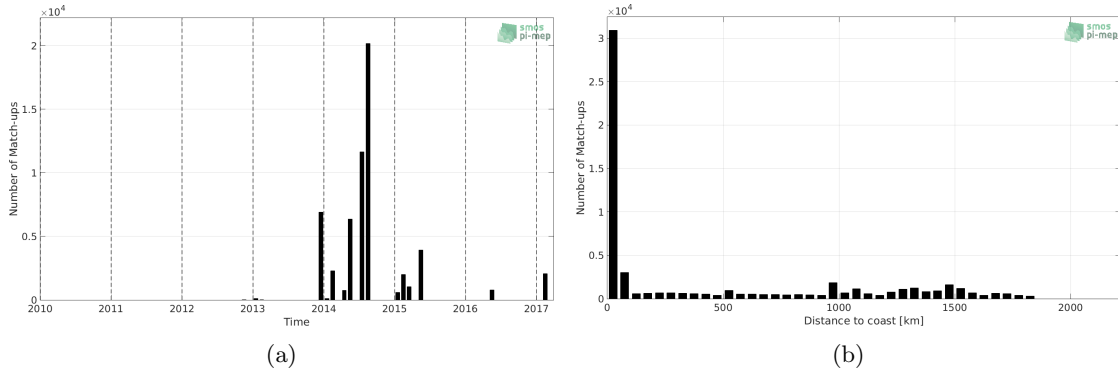
Figure 1: Number of match-ups between TSG (GOSUD-Sailing-ship) and SMOS L3 v2 - 9-Days (BEC) SSS as a function of time (a) and as function of the distance to coast (b) over the Amazon and Orinoco river plumes Pi-MEP region and for the full satellite product period.
