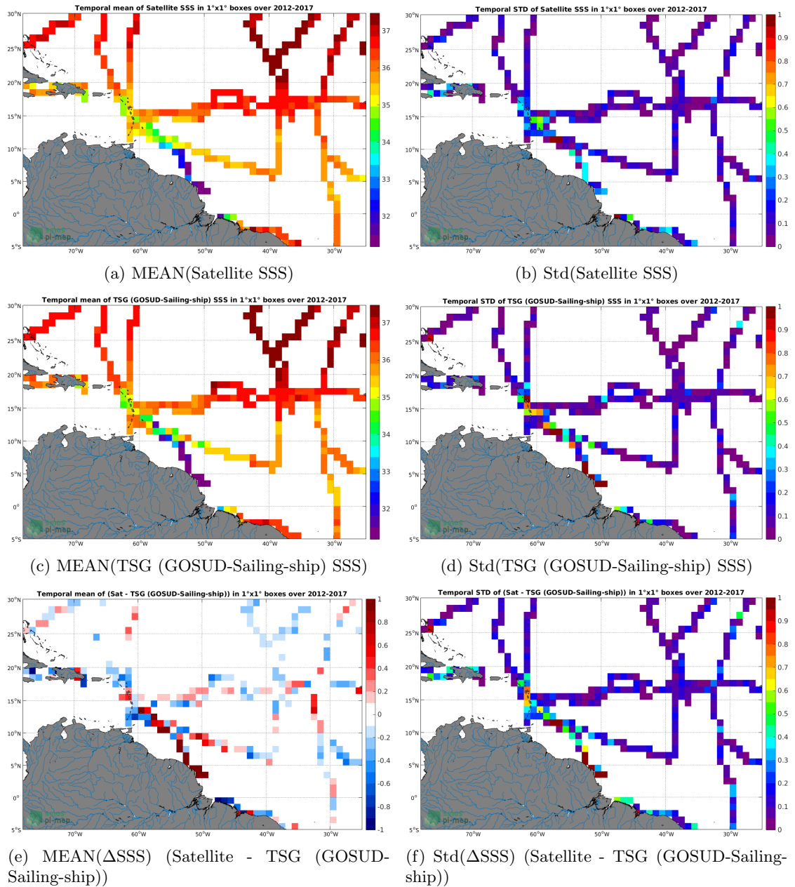
Figure 6: Temporal mean (left) and Std (right) of SSS from SMOS L3 v2 - 9-Days (BEC) (top), TSG (GOSUD-Sailing-ship) (middle), and of \Delta SSS (Satellite - TSG (GOSUD-Sailing-ship)). Only match-up pairs are used to generate these maps.
