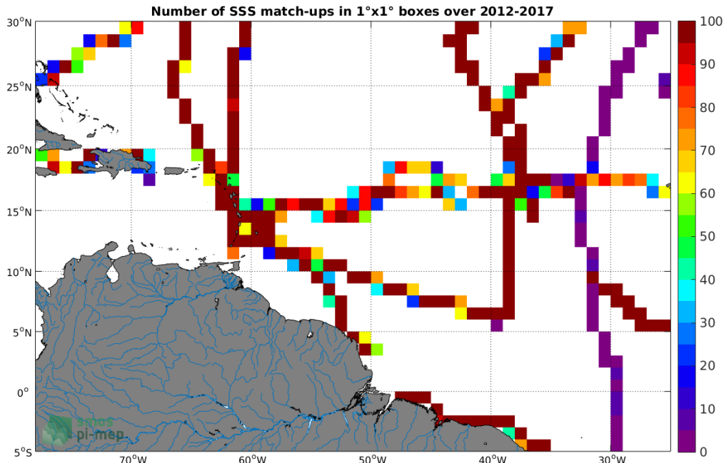
Figure 4: Number of SSS match-ups between TSG (GOSUD-Sailing-ship) SSS and the SMOS L3 v2 - 9-Days (BEC) SSS product for the Amazon and Orinoco river plumes Pi-MEP region over 1°x1° boxes and for the full satellite product period.
