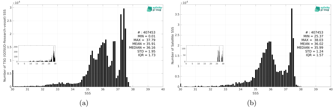
Figure 3: Histograms of SSS from TSG (GOSUD-Research-vessel) (a) and SMOS SSS L3 v2 - 9-Days (BEC) (b) considering all match-up pairs per bins of 0.1 over the Amazon and Orinoco river plumes Pi-MEP region and for the full satellite product period.
