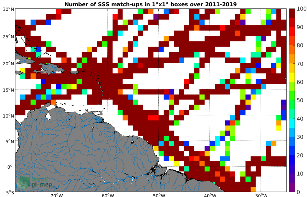
Figure 4: Number of SSS match-ups between TSG (GOSUD-Research-vessel) SSS and the SMOS SSS L3 v2 - 9-Days (BEC) SSS product for the Amazon and Orinoco river plumes Pi-MEP region over 1°x1° boxes and for the full satellite period.
