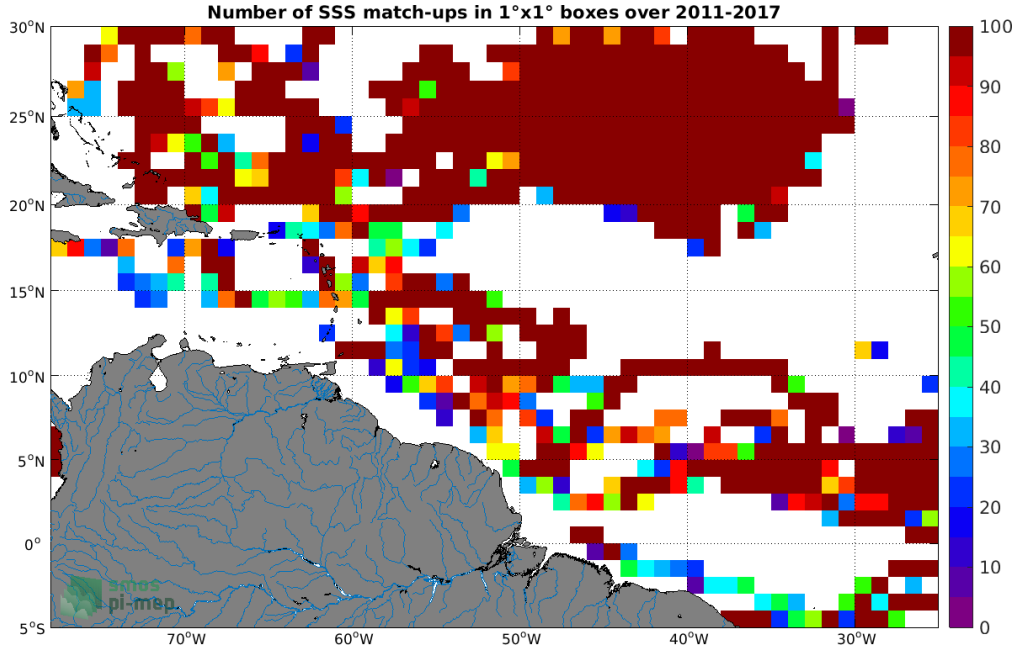
Figure 3: Number of SSS match-ups between Surface drifters SSS and the SMOS SSS L3 v2 - 9-Days (BEC) SSS product for the Amazon and Orinoco river plumes Pi-MEP region over 1°x1° boxes and for the full satellite product period.
