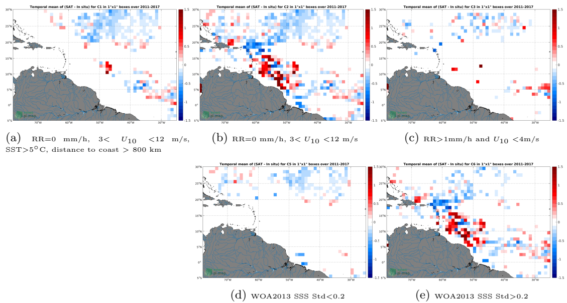
Figure 11: Temporal mean gridded over spatial boxes of size 1°x1° of \Delta SSS (SMOS SSS L3 v2 - 9-Days (BEC) - Surface drifters) for 5 different subdatasets corresponding to: RR=0 mm/h, 3 < U_{10} < 12 m/s, SST > 5°C, distance to coast > 800 km (a), RR=0 mm/h, 3 < U_{10} < 12 m/s (b), RR > 1mm/h and U_{10} < 4 m/s (c), WOA2013 SSS Std < 0.2 (d), WOA2013 SSS Std > 0.2 (e).
