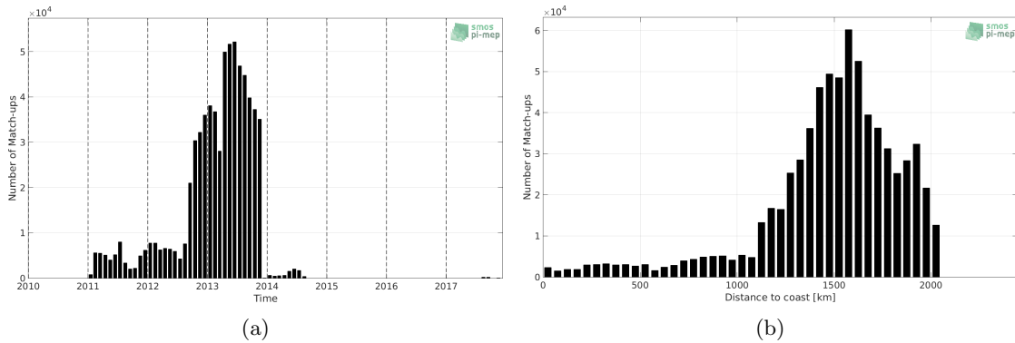
Figure 1: Number of match-ups between Surface drifters and SMOS L3 v2 - 9-Days (BEC) SSS as a function of time (a) and as function of the distance to coast (b) over the Amazon and Orinoco river plumes Pi-MEP region and for the full satellite product period.
