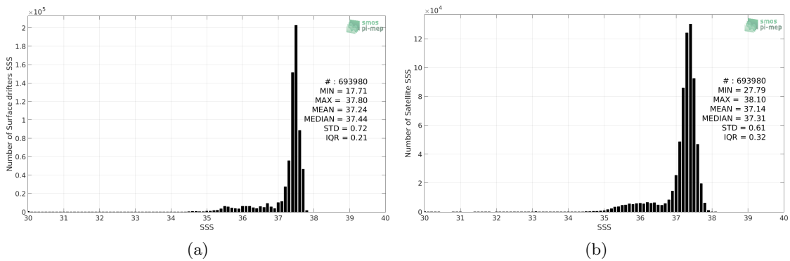
Figure 2: Histograms of SSS from Surface drifters (a) and SMOS L3 v2 - 9-Days (BEC) (b) considering all match-up pairs per bins of 0.1 over the Amazon and Orinoco river plumes Pi-MEP region and for the full satellite product period.
