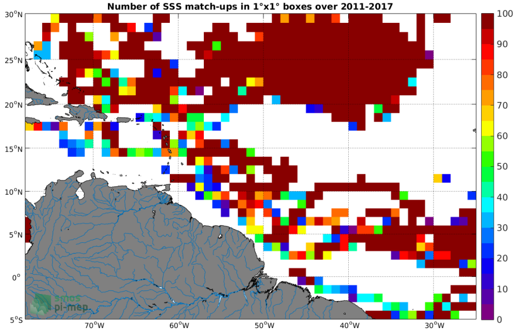
Figure 3: Number of SSS match-ups between Surface drifters SSS and the SMOS L3 v2 - 9-Days (BEC) SSS product for the Amazon and Orinoco river plumes Pi-MEP region over 1°x1° boxes and for the full satellite product period.
