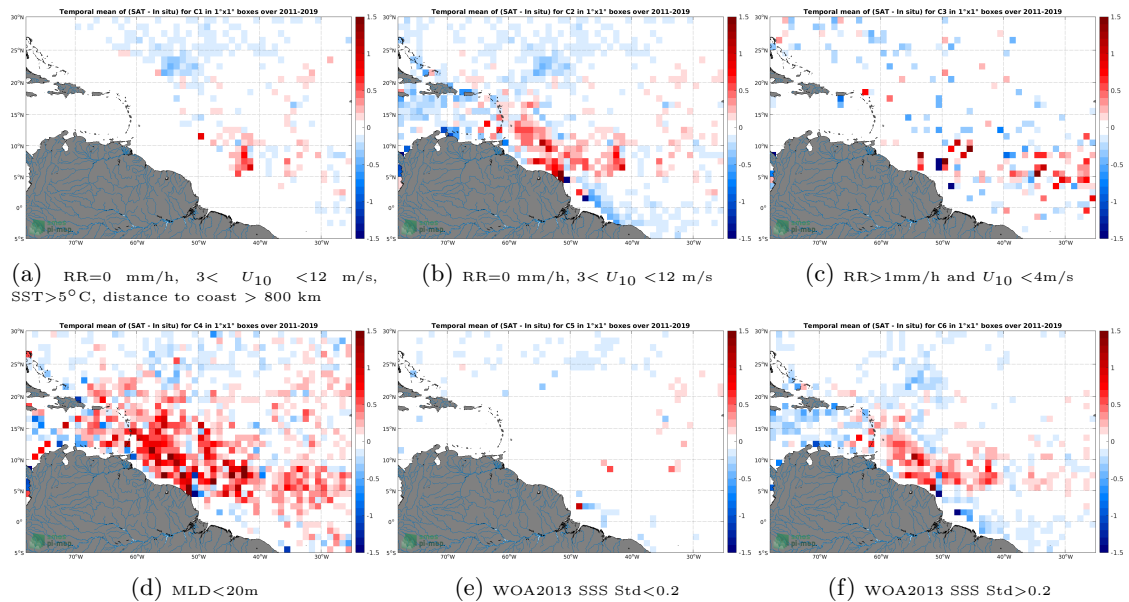
Figure 12: Temporal mean gridded over spatial boxes of size 1°x1° of \Delta SSS (SMOS SSS L3 v2 - 9-Days (BEC) - Argo) for 6 different subdatasets corresponding to:RR=0 mm/h, 3 < U_{10} < 12 m/s, SST>5°C, distance to coast > 800 km (a), RR=0 mm/h, 3 < U_{10} < 12 m/s (b), RR>1mm/h and U_{10} < 4 m/s (c),MLD<20m (d),WOA2013 SSS Std<0.2 (e),WOA2013 SSS Std>0.2 (f).
