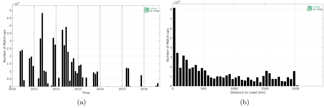
Figure 1: Number of match-ups between TSG-SAMOS and SMOS-L3-BEC-OA-V1-9DAYS-0.25DEG SSS as a function of time (a) and as function of the distance to coast (b) over the Amazon and Orinoco river plumes Pi-MEP region and for the full satellite product period.
