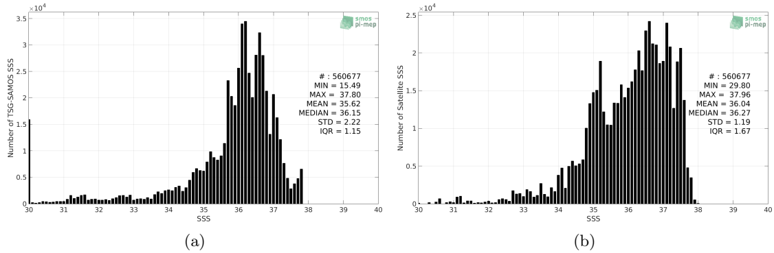
Figure 2: Histograms of SSS from TSG-SAMOS (a) and SMOS-L3-BEC-OA-V1-9DAYS-0.25DEG (b) considering all match-up pairs per bins of 0.1 over the Amazon and Orinoco river plumes Pi-MEP region and for the full satellite product period.
