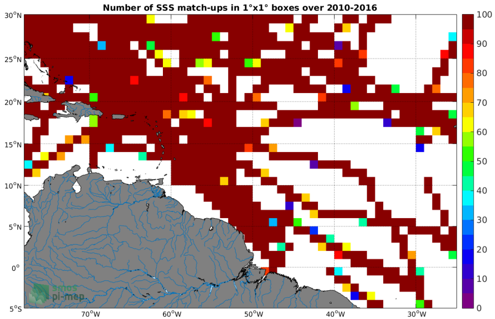
Figure 4: Number of SSS match-ups between TSG-SAMOS SSS and the SMOS-L3-BEC-OA-V1-9DAYS-0.25DEG SSS product for the Amazon and Orinoco river plumes Pi-MEP region over 1°x1° boxes and for the full satellite product period.
