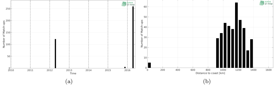
Figure 1: Number of match-ups between TSG-POLARSTERN and SMOS-L3-BEC-OA-V1-9DAYS-0.25DEG SSS as a function of time (a) and as function of the distance to coast (b) over the Amazon and Orinoco river plumes Pi-MEP region and for the full satellite product period.
