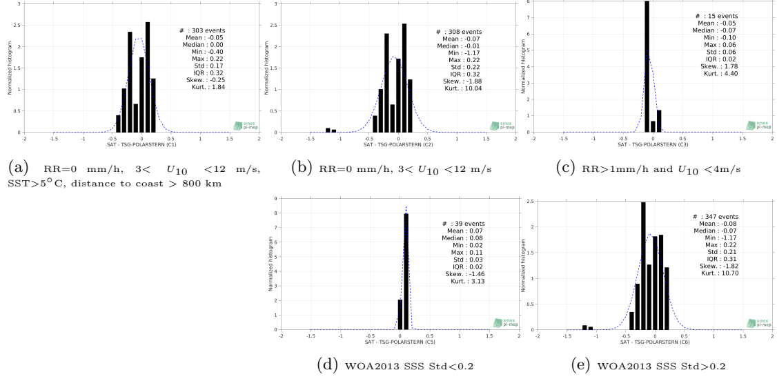
Figure 13: Normalized histogram of \Delta SSS (SMOS-L3-BEC-OA-V1-9DAYS-0.25DEG - TSG-POLARSTERN) for 5 different subdatasets corresponding to: RR=0 mm/h, 3 < U_{10} < 12 m/s, SST>5°C, distance to coast > 800 km (a), RR=0 mm/h, 3 < U_{10} < 12 m/s (b), RR>1mm/h and U_{10} < 4 m/s (c), WOA2013 SSS Std<0.2 (d), WOA2013 SSS Std>0.2 (e).
