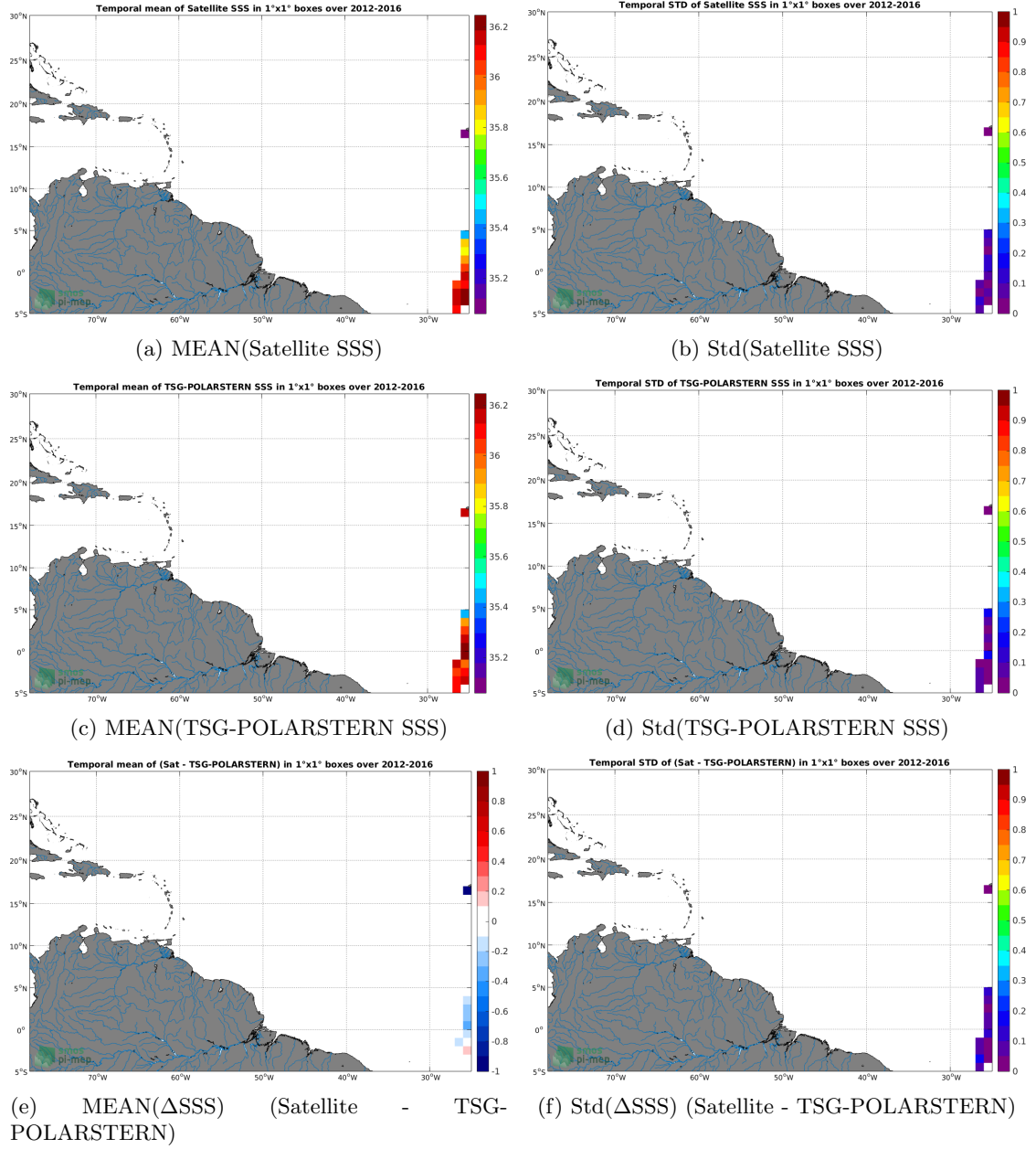
Figure 6: Temporal mean (left) and Std (right) of SSS from SMOS-L3-BEC-OA-V1-9DAYS-0.25DEG (top), TSG-POLARSTERN (middle), and of \Delta SSS (Satellite - TSG-POLARSTERN). Only match-up pairs are used to generate these maps.
