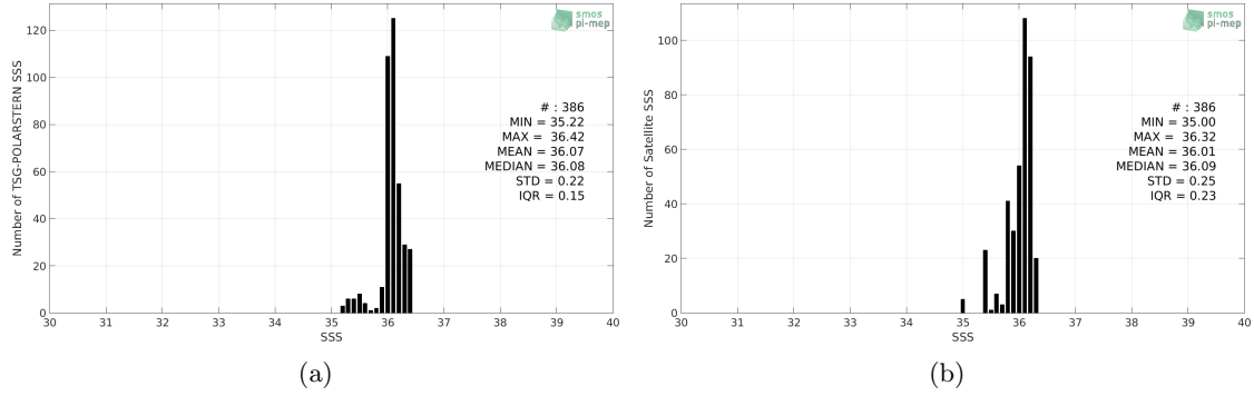
Figure 2: Histograms of SSS from TSG-POLARSTERN (a) and SMOS-L3-BEC-OA-V1-9DAYS-0.25DEG (b) considering all match-up pairs per bins of 0.1 over the Amazon and Orinoco river plumes Pi-MEP region and for the full satellite product period.
