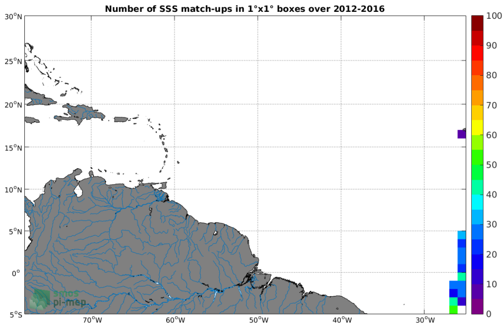
Figure 4: Number of SSS match-ups between TSG-POLARSTERN SSS and the SMOS-L3-BEC-OA-V1-9DAYS-0.25DEG SSS product for the Amazon and Orinoco river plumes Pi-MEP region over 1^\circ \times 1^\circ boxes and for the full satellite product period.
