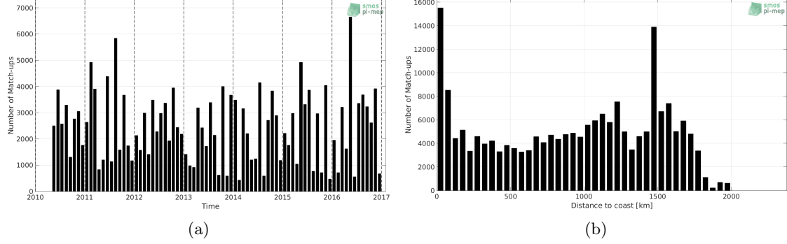
Figure 1: Number of match-ups between TSG-LEGOS-DM and SMOS-L3-BEC-OA-V1-9DAYS-0.25DEG SSS as a function of time (a) and as function of the distance to coast (b) over the Amazon and Orinoco river plumes Pi-MEP region and for the full satellite product period.
