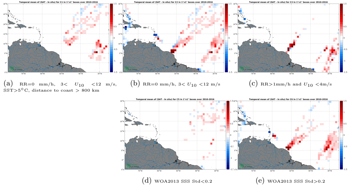
Figure 12: Temporal mean gridded over spatial boxes of size 1^\circ \times 1^\circ of \Delta SSS (SMOS-L3-BEC-OA-V1-9DAYS-0.25DEG - TSG-LEGOS-DM) for 5 different subdatasets corresponding to: RR=0 mm/h, 3 < U_{10} < 12 m/s, SST > 5^\circ C , distance to coast > 800 km (a), RR=0 mm/h, 3 < U_{10} < 12 m/s (b), RR > 1 mm/h and U_{10} < 4 m/s (c), WOA2013 SSS Std < 0.2 (d), WOA2013 SSS Std > 0.2 (e).
