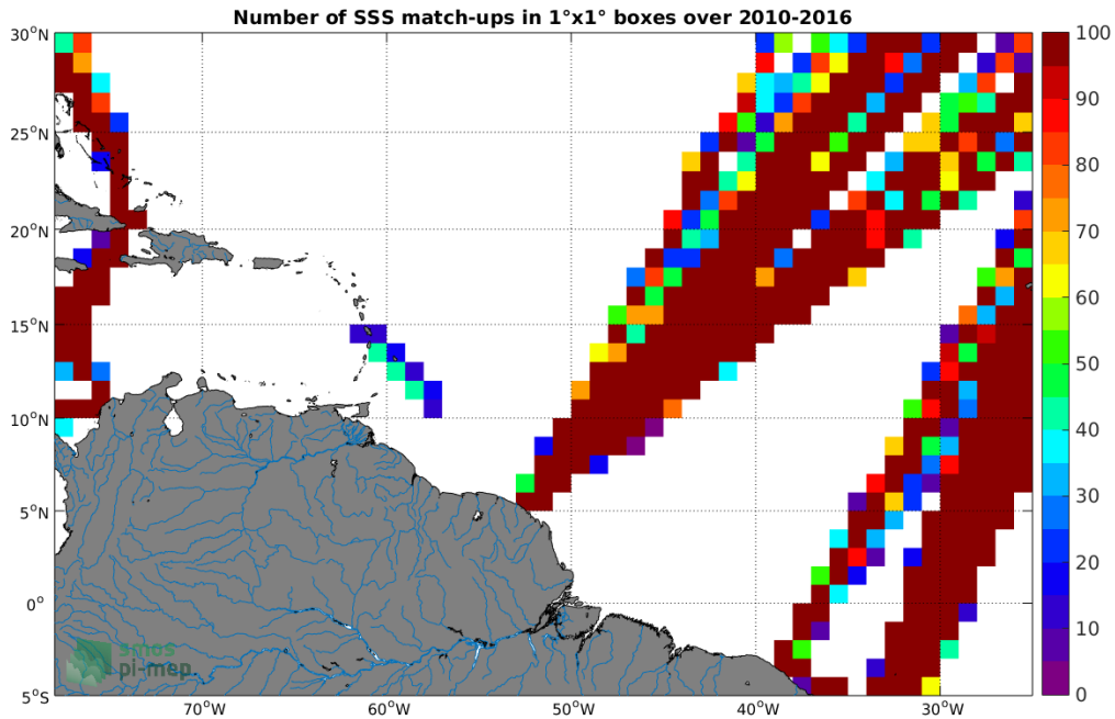
Figure 4: Number of SSS match-ups between TSG-LEGOS-DM SSS and the SMOS-L3-BEC-OA-V1-9DAYS-0.25DEG SSS product for the Amazon and Orinoco river plumes Pi-MEP region over 1^\circ \times 1^\circ boxes and for the full satellite product period.
