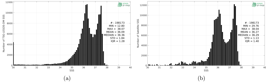
Figure 2: Histograms of SSS from TSG-LEGOS-DM (a) and SMOS-L3-BEC-OA-V1-9DAYS-0.25DEG (b) considering all match-up pairs per bins of 0.1 over the Amazon and Orinoco river plumes Pi-MEP region and for the full satellite product period.
