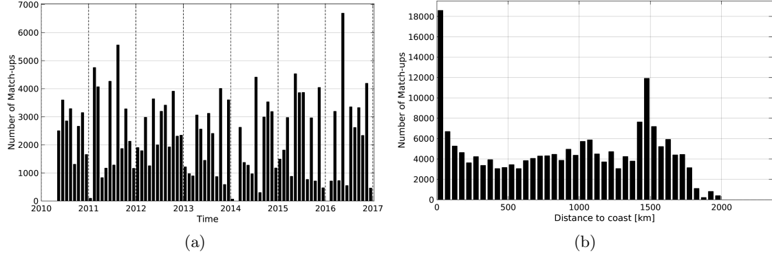
Figure 1: Number of match-ups between TSG-LEGOS-DM and SMOS-L3-BEC-OA-V1-9DAYS-0.25DEG SSS as a function of time (a) and as function of the distance to coast (b) over the Amazon and Orinoco river plumes Pi-MEP region and for the full satellite product period.
