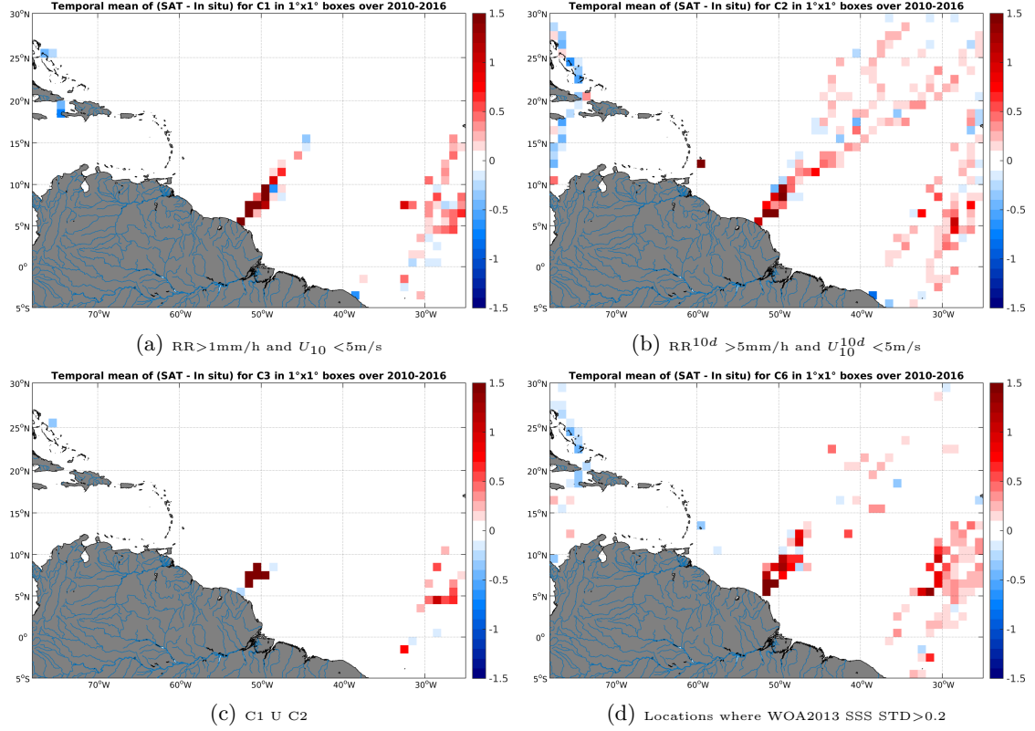
Figure 12: Temporal mean gridded over spatial boxes of size 1^\circ \times 1^\circ of \Delta SSS (SMOS-L3-BEC-OA-V1-9DAYS-0.25DEG - TSG-LEGOS-DM) for 4 different subdatasets corresponding to: RR > 1 mm/h and U_{10} < 5 m/s (a), RR ^{10d} > 5 mm/h and U_{10}^{10d} < 5 m/s (b), C1 U C2 (c), Locations where WOA2013 SSS STD > 0.2 (d).
