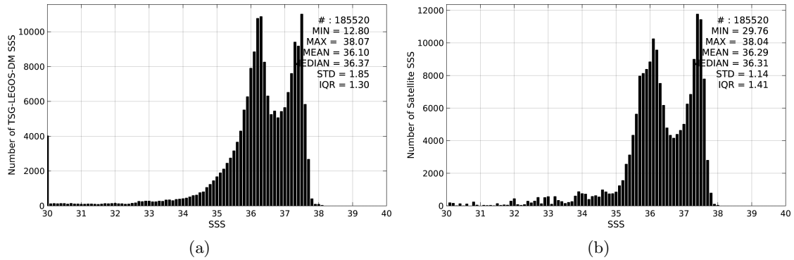
Figure 2: Histograms of SSS from TSG-LEGOS-DM (a) and SMOS-L3-BEC-OA-V1-9DAYS-0.25DEG (b) considering all match-up pairs per bins of 0.1 over the Amazon and Orinoco river plumes Pi-MEP region and for the full satellite product period.
