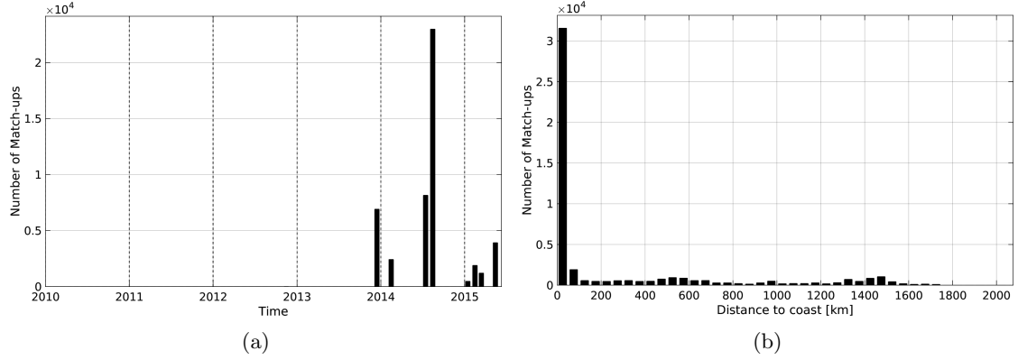
Figure 1: Number of match-ups between TSG-GOSUD-Sailing-ship and SMOS-L3-BEC-OA-V1-9DAYS-0.25DEG SSS as a function of time (a) and as function of the distance to coast (b) over the Amazon and Orinoco river plumes Pi-MEP region and for the full satellite product period.
