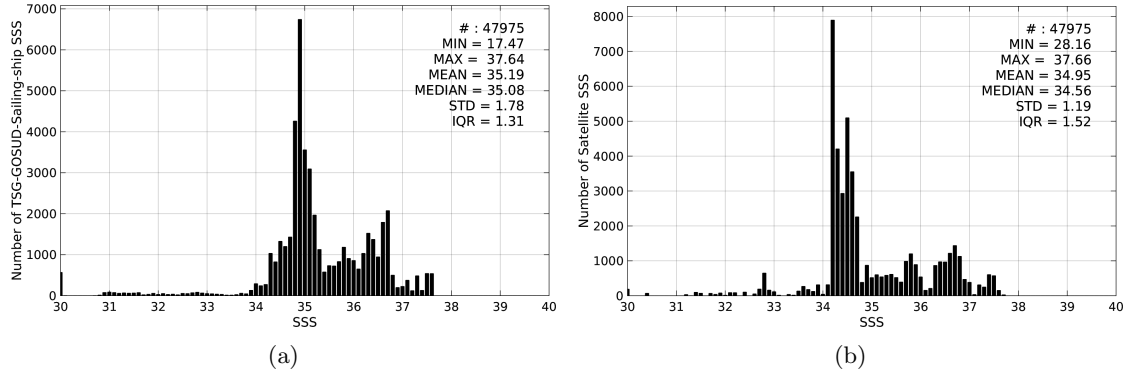
Figure 2: Histograms of SSS from TSG-GOSUD-Sailing-ship (a) and SMOS-L3-BEC-OA-V1-9DAYS-0.25DEG (b) considering all match-up pairs per bins of 0.1 over the Amazon and Orinoco river plumes Pi-MEP region and for the full satellite product period.
