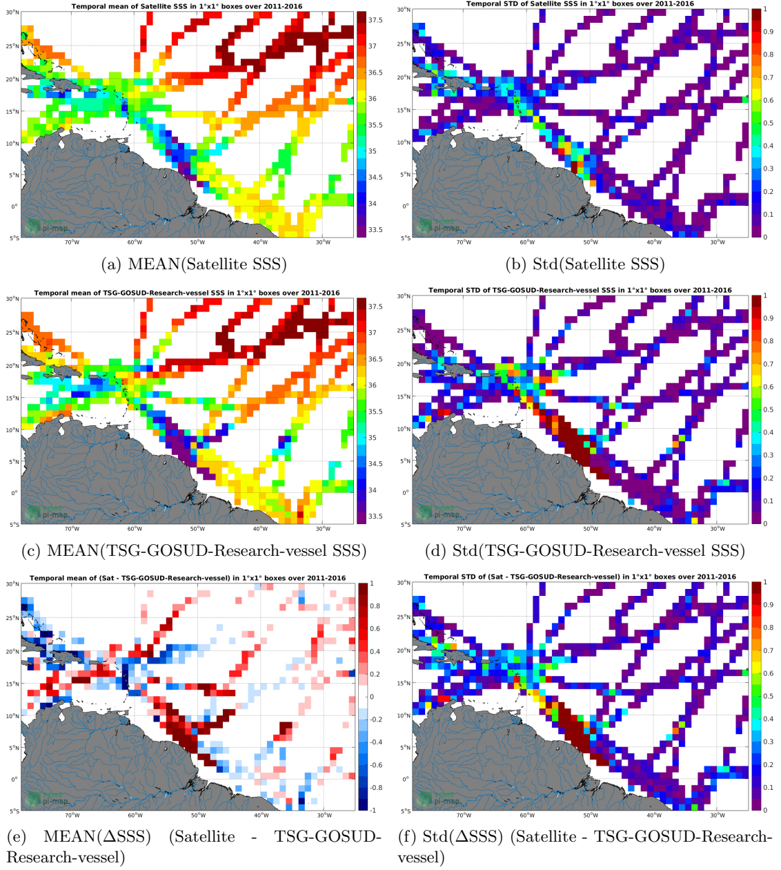
Figure 6: Temporal mean (left) and Std (right) of SSS from SMOS-L3-BEC-OA-V1-9DAYS-0.25DEG (top), TSG-GOSUD-Research-vessel (middle), and of \Delta SSS (Satellite - TSG-GOSUD-Research-vessel). Only match-up pairs are used to generate these maps.
