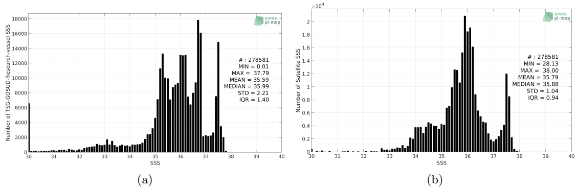
Figure 2: Histograms of SSS from TSG-GOSUD-Research-vessel (a) and SMOS-L3-BEC-OA-V1-9DAYS-0.25DEG (b) considering all match-up pairs per bins of 0.1 over the Amazon and Orinoco river plumes Pi-MEP region and for the full satellite product period.
