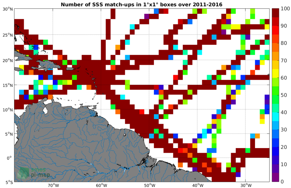
Figure 4: Number of SSS match-ups between TSG-GOSUD-Research-vessel SSS and the SMOS-L3-BEC-OA-V1-9DAYS-0.25DEG SSS product for the Amazon and Orinoco river plumes Pi-MEP region over 1^\circ \times 1^\circ boxes and for the full satellite product period.
