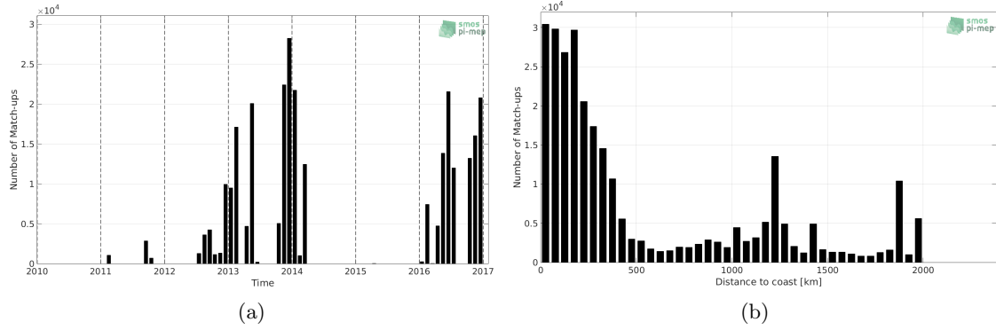
Figure 1: Number of match-ups between TSG-GOSUD-Research-vessel and SMOS-L3-BEC-OA-V1-9DAYS-0.25DEG SSS as a function of time (a) and as function of the distance to coast (b) over the Amazon and Orinoco river plumes Pi-MEP region and for the full satellite product period.
