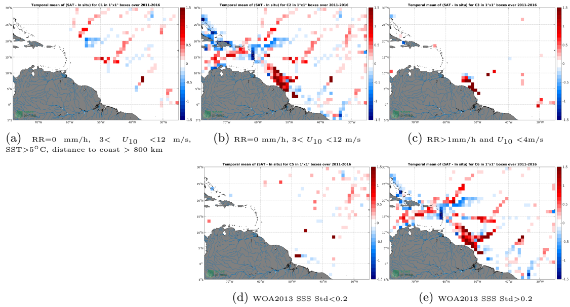
Figure 12: Temporal mean gridded over spatial boxes of size 1^\circ \times 1^\circ of \Delta SSS (SMOS-L3-BEC-OA-V1-9DAYS-0.25DEG - TSG-GOSUD-Research-vessel) for 5 different subdatasets corresponding to: RR=0 mm/h, 3 < U_{10} < 12 m/s, SST > 5^\circ C , distance to coast > 800 km (a), RR=0 mm/h, 3 < U_{10} < 12 m/s (b), RR > 1 mm/h and U_{10} < 4 m/s (c), WOA2013 SSS Std < 0.2 (d), WOA2013 SSS Std > 0.2 (e).
