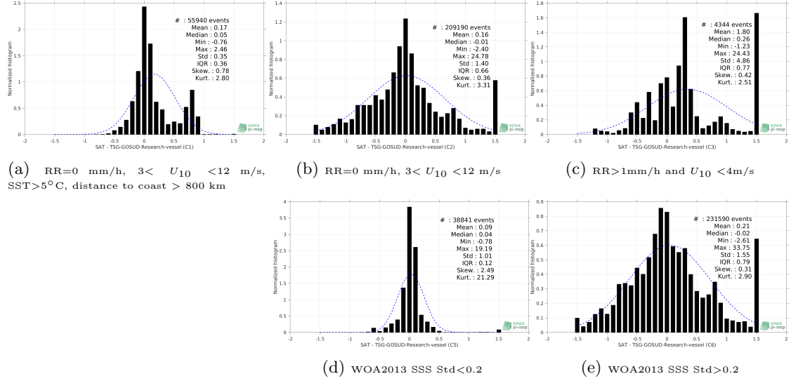
Figure 13: Normalized histogram of \Delta SSS (SMOS-L3-BEC-OA-V1-9DAYS-0.25DEG - TSG-GOSUD-Research-vessel) for 5 different subdatasets corresponding to: RR=0 mm/h, 3 < U_{10} < 12 m/s, SST>5°C, distance to coast > 800 km (a), RR=0 mm/h, 3 < U_{10} < 12 m/s (b), RR>1mm/h and U_{10} < 4 m/s (c), WOA2013 SSS Std<0.2 (d), WOA2013 SSS Std>0.2 (e).
