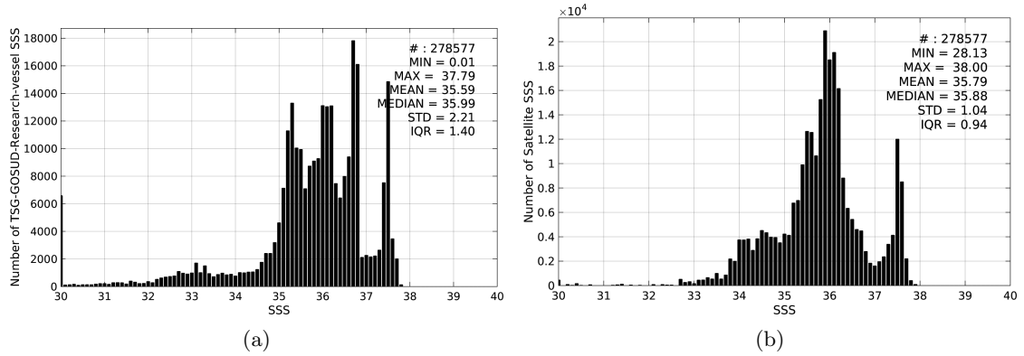
Figure 2: Histograms of SSS from TSG-GOSUD-Research-vessel (a) and SMOS-L3-BEC-OA-V1-9DAYS-0.25DEG (b) considering all match-up pairs per bins of 0.1 over the Amazon and Orinoco river plumes Pi-MEP region and for the full satellite product period.
