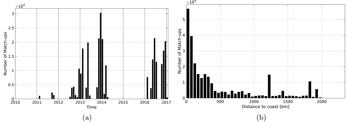
Figure 1: Number of match-ups between TSG-GOSUD-Research-vessel and SMOS-L3-BEC-OA-V1-9DAYS-0.25DEG SSS as a function of time (a) and as function of the distance to coast (b) over the Amazon and Orinoco river plumes Pi-MEP region and for the full satellite product period.
