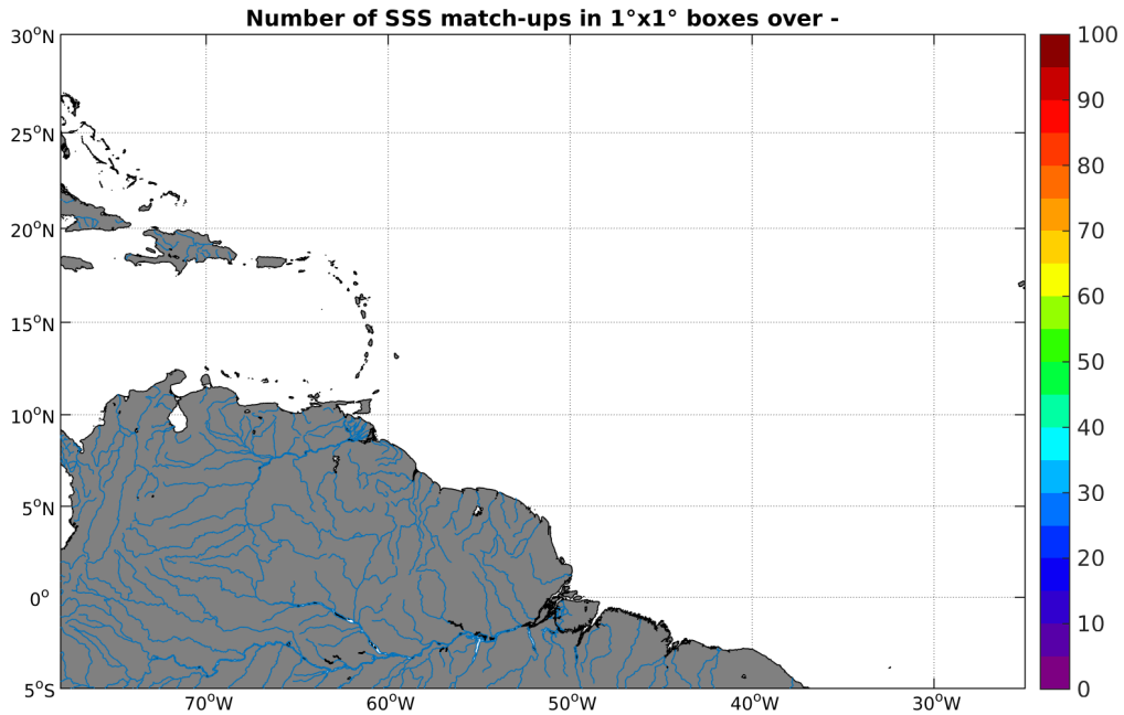
Figure 4: Number of SSS match-ups between Sea mammals SSS and the SMOS-L3-BEC-OA-V1-9DAYS-0.25DEG SSS product for the Amazon and Orinoco river plumes Pi-MEP region over 1°x1° boxes and for the full satellite product period.
