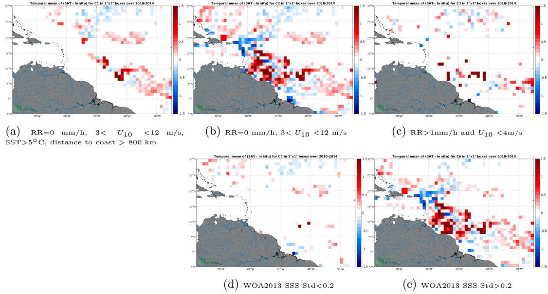
Figure 11: Temporal mean gridded over spatial boxes of size 1^\circ \times 1^\circ of \Delta SSS (SMOS-L3-BEC-OA-V1-9DAYS-0.25DEG - Surface drifters) for 5 different subdatasets corresponding to: RR=0 mm/h, 3 < U_{10} < 12 m/s, SST > 5^\circ C , distance to coast > 800 km (a), RR=0 mm/h, 3 < U_{10} < 12 m/s (b), RR > 1 mm/h and U_{10} < 4 m/s (c), WOA2013 SSS Std < 0.2 (d), WOA2013 SSS Std > 0.2 (e).
