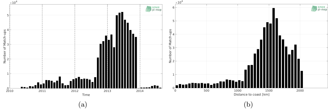
Figure 1: Number of match-ups between Surface drifters and SMOS-L3-BEC-OA-V1-9DAYS-0.25DEG SSS as a function of time (a) and as function of the distance to coast (b) over the Amazon and Orinoco river plumes Pi-MEP region and for the full satellite product period.
