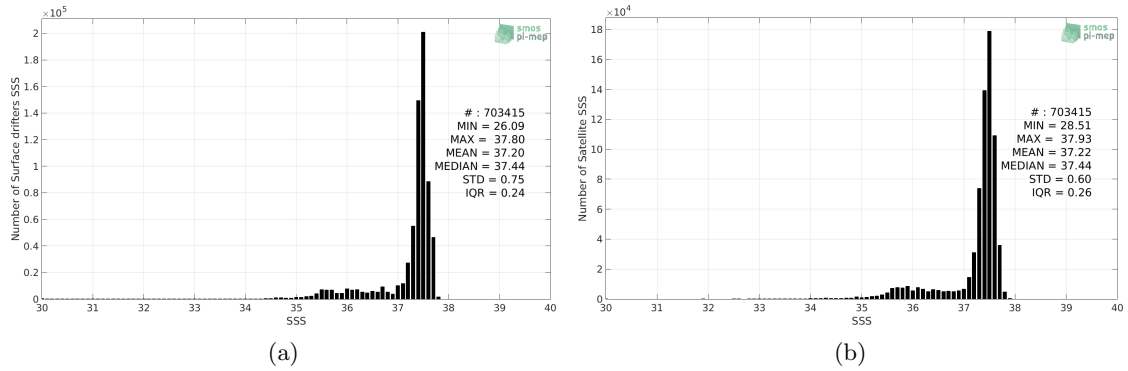
Figure 2: Histograms of SSS from Surface drifters (a) and SMOS-L3-BEC-OA-V1-9DAYS-0.25DEG (b) considering all match-up pairs per bins of 0.1 over the Amazon and Orinoco river plumes Pi-MEP region and for the full satellite product period.
