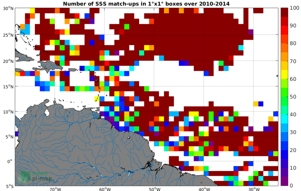
Figure 3: Number of SSS match-ups between Surface drifters SSS and the SMOS-L3-BEC-OA-V1-9DAYS-0.25DEG SSS product for the Amazon and Orinoco river plumes Pi-MEP region over 1^\circ \times 1^\circ boxes and for the full satellite product period.
