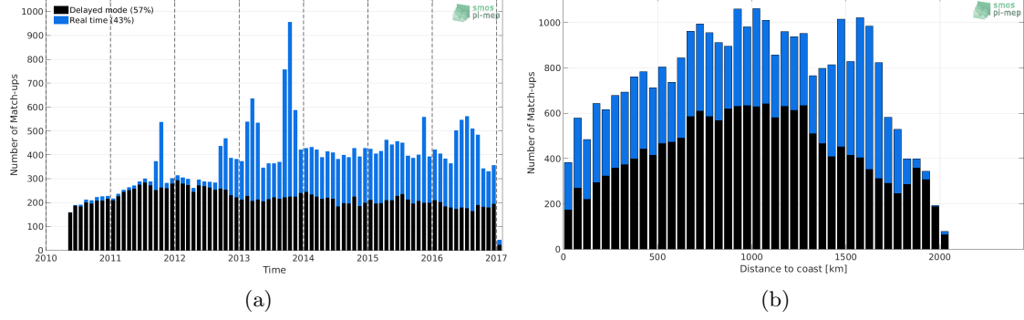
Figure 1: Number of match-ups between Argo and SMOS-L3-BEC-OA-V1-9DAYS-0.25DEG SSS as a function of time (a) and as function of the distance to coast (b) over the Amazon and Orinoco river plumes Pi-MEP region and for the full satellite product period.
