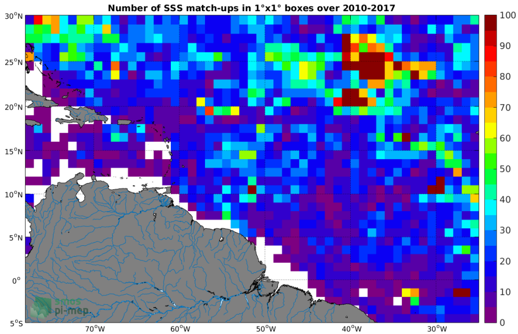
Figure 4: Number of SSS match-ups between Argos SSS and the SMOS-L3-BEC-OA-V1-9DAYS-0.25DEG SSS product for the Amazon and Orinoco river plumes Pi-MEP region over 1°x1° boxes and for the full satellite product period.
