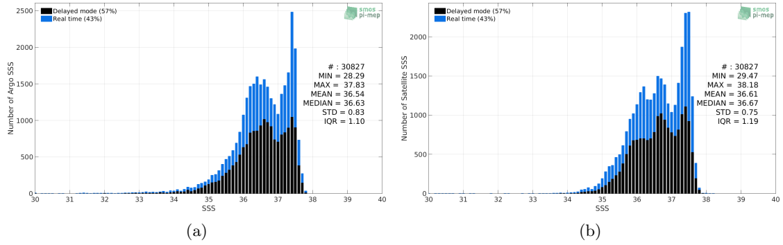
Figure 2: Histograms of SSS from Argo (a) and SMOS-L3-BEC-OA-V1-9DAYS-0.25DEG (b) considering all match-up pairs per bins of 0.1 over the Amazon and Orinoco river plumes Pi-MEP region and for the full satellite product period.
