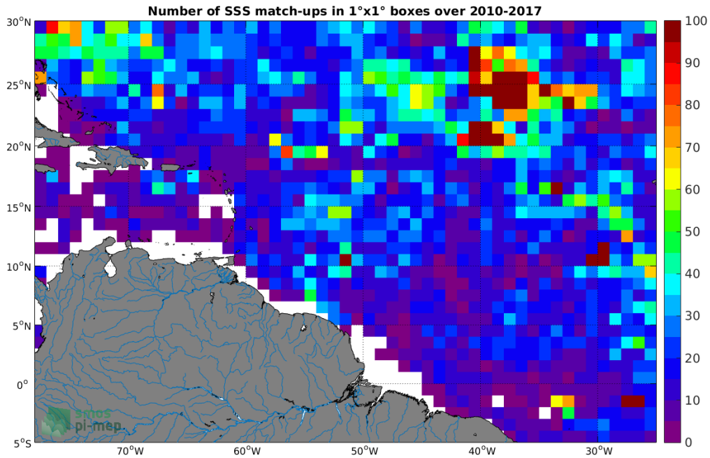
Figure 4: Number of SSS match-ups between Argo SSS and the SMOS-L3-BEC-OA-V1-9DAYS-0.25DEG SSS product for the Amazon and Orinoco river plumes Pi-MEP region over 1^\circ \times 1^\circ boxes and for the full satellite product period.
