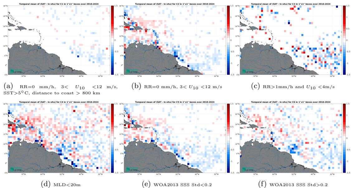
Figure 14: Temporal mean gridded over spatial boxes of size 1^\circ \times 1^\circ of \Delta SSS (SMOS SSS L2-AVERAGED v700 (ESA) - Argo) for 6 different subdatasets corresponding to:RR=0 mm/h, 3 < U_{10} < 12 m/s, SST >5^\circ C, distance to coast > 800 km (a), RR=0 mm/h, 3 < U_{10} < 12 m/s (b), RR >1 mm/h and U_{10} < 4 m/s (c),MLD <20 m (d),WOA2013 SSS Std <0.2 (e),WOA2013 SSS Std >0.2 (f).
