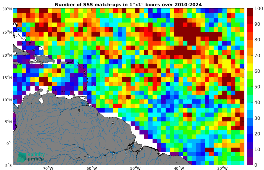
Figure 5: Number of SSS match-ups between Argo SSS and the SMOS SSS L2-AVERAGED v700 (ESA) SSS product for the Amazon and Orinoco river plumes Pi-MEP region over 1^\circ \times 1^\circ boxes and for the full satellite product period.
