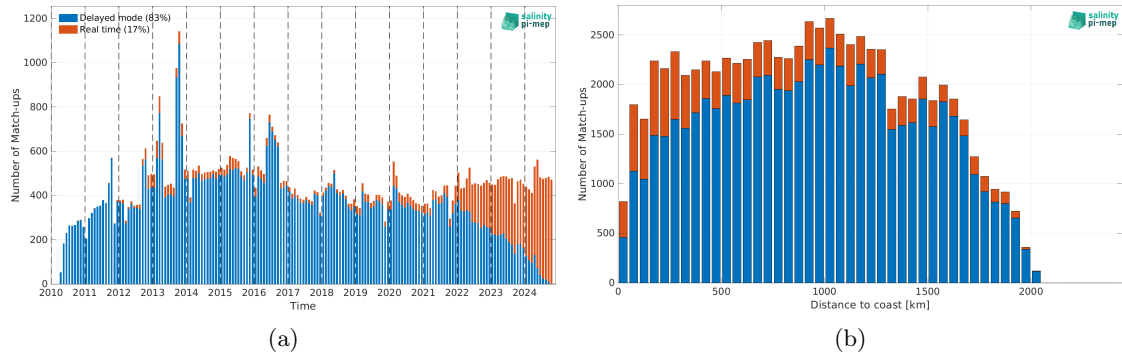
Figure 2: Number of match-ups between Argo and SMOS SSS L2-AVERAGED v700 (ESA) SSS as a function of time (a) and as function of the distance to coast (b) over the Amazon and Orinoco river plumes Pi-MEP region and for the full satellite product period.
