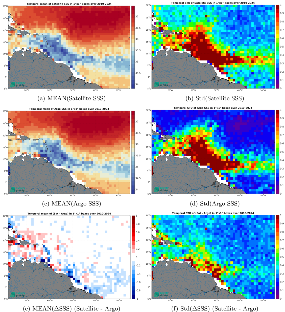
Figure 7: Temporal mean (left) and Std (right) of SSS from SMOS SSS L2-AVERAGED v700 (ESA) (top), Argo (middle), and of \Delta SSS (Satellite - Argo). Only match-up pairs are used to generate these maps.
