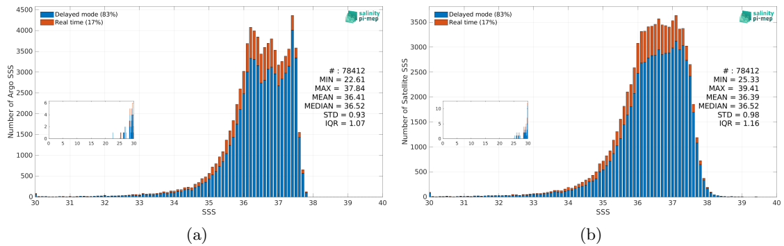
Figure 3: Histograms of SSS from Argo (a) and SMOS SSS L2-AVERAGED v700 (ESA) (b) considering all match-up pairs per bins of 0.1 over the Amazon and Orinoco river plumes Pi-MEP region and for the full satellite product period.
