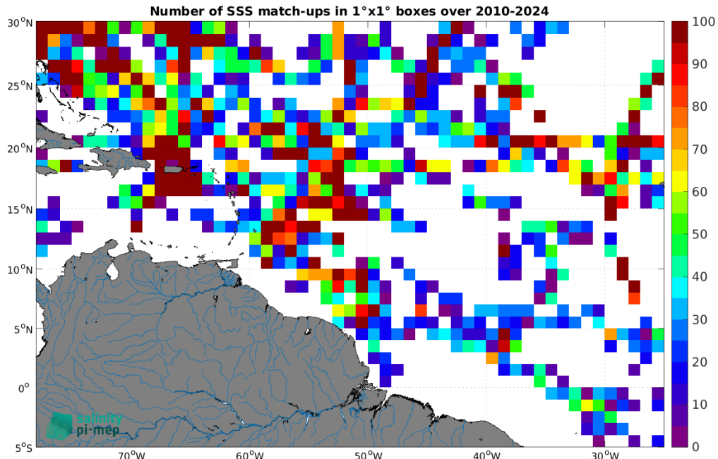
Figure 5: Number of SSS match-ups between TSG (SAMOS) SSS and the SMOS SSS L2 v700 (ESA) SSS product for the Amazon and Orinoco river plumes Pi-MEP region over 1^\circ \times 1^\circ boxes and for the full satellite product period.
