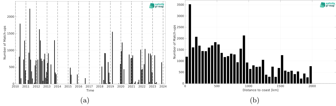
Figure 2: Number of match-ups between TSG (SAMOS) and SMOS SSS L2 v700 (ESA) SSS as a function of time (a) and as function of the distance to coast (b) over the Amazon and Orinoco river plumes Pi-MEP region and for the full satellite product period.
