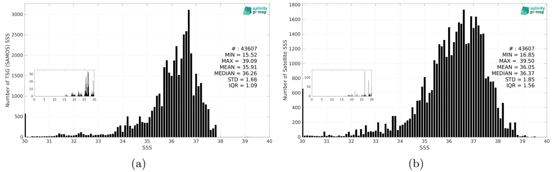
Figure 3: Histograms of SSS from TSG (SAMOS) (a) and SMOS SSS L2 v700 (ESA) (b) considering all match-up pairs per bins of 0.1 over the Amazon and Orinoco river plumes Pi-MEP region and for the full satellite product period.
