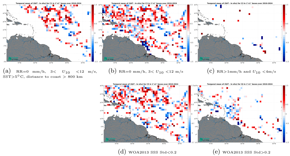
Figure 14: Temporal mean gridded over spatial boxes of size 1^\circ \times 1^\circ of \Delta SSS (SMOS SSS L2 v700 (ESA) - TSG (SAMOS)) for 5 different subdatasets corresponding to: RR=0 mm/h, 3 < U_{10} < 12 m/s, SST > 5^\circ C , distance to coast > 800 km (a), RR=0 mm/h, 3 < U_{10} < 12 m/s (b), RR > 1 mm/h and U_{10} < 4 m/s (c), WOA2013 SSS Std < 0.2 (d), WOA2013 SSS Std > 0.2 (e).
