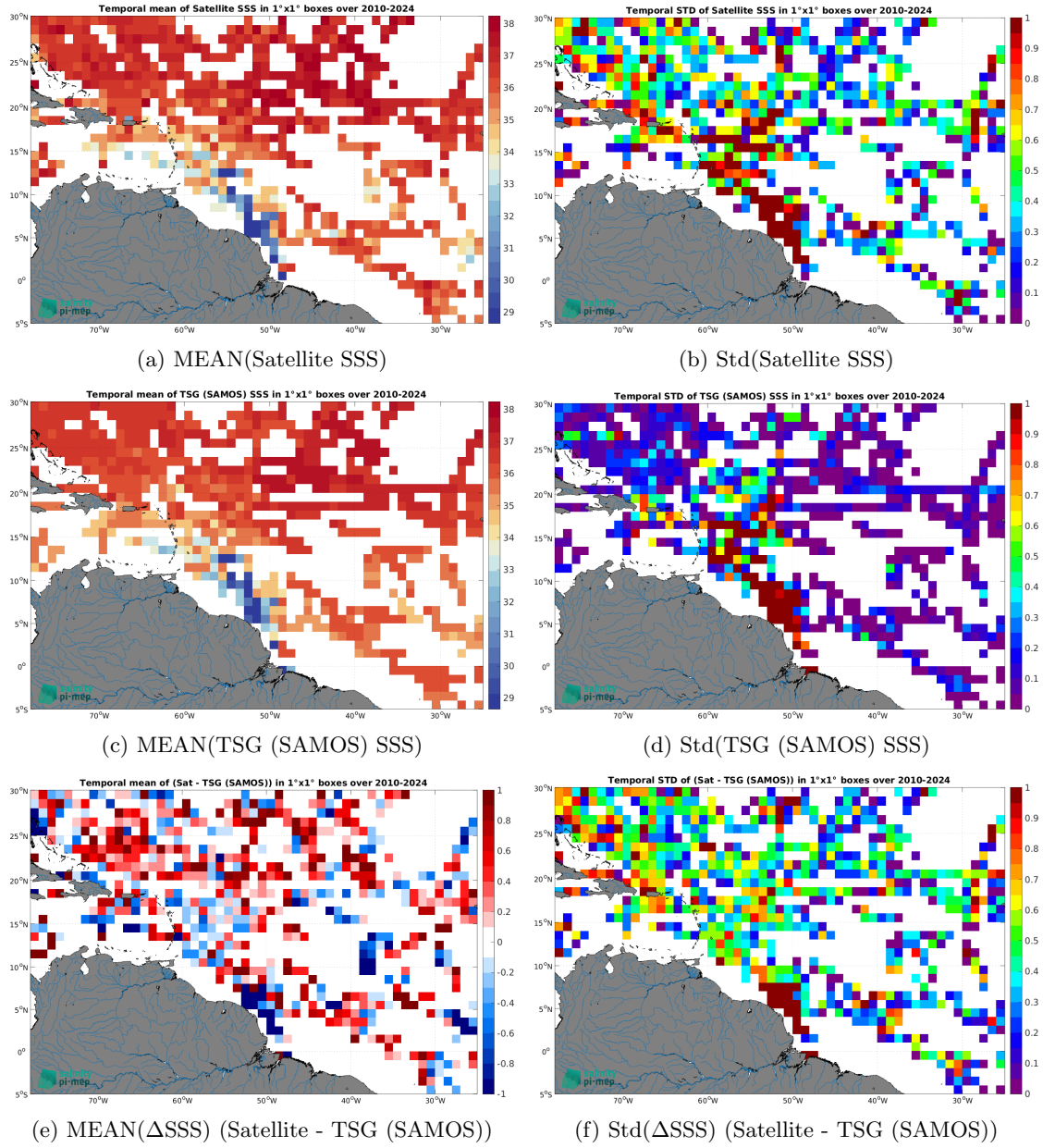
Figure 7: Temporal mean (left) and Std (right) of SSS from SMOS SSS L2 v700 (ESA) (top), TSG (SAMOS) (middle), and of \Delta SSS (Satellite - TSG (SAMOS)). Only match-up pairs are used to generate these maps.
