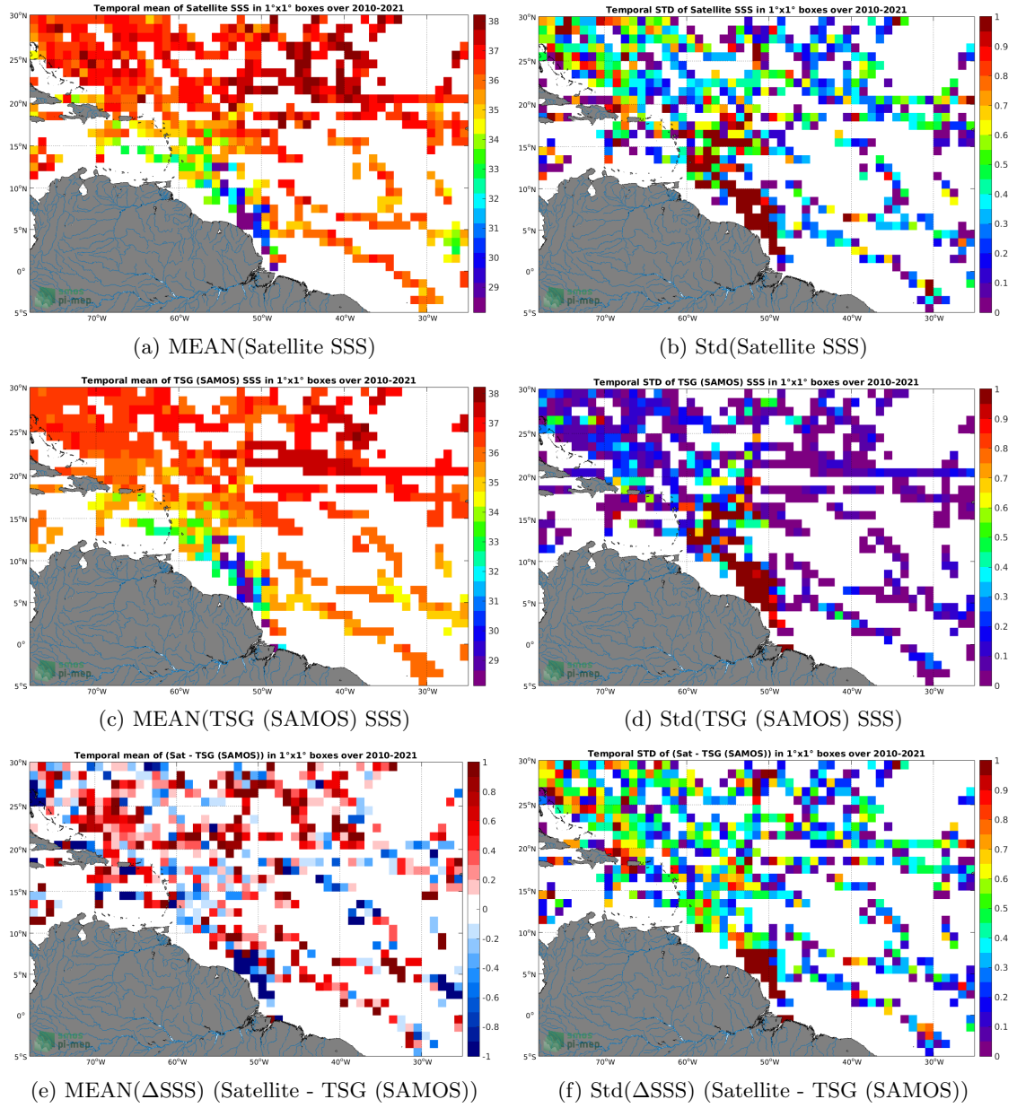
Figure 6: Temporal mean (left) and Std (right) of SSS from SMOS SSS L2 v700 (ESA) (top), TSG (SAMOS) (middle), and of \Delta SSS (Satellite - TSG (SAMOS)). Only match-up pairs are used to generate these maps.
