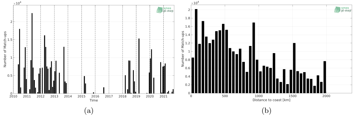
Figure 1: Number of match-ups between TSG (SAMOS) and SMOS SSS L2 v700 (ESA) SSS as a function of time (a) and as function of the distance to coast (b) over the Amazon and Orinoco river plumes Pi-MEP region and for the full satellite product period.
