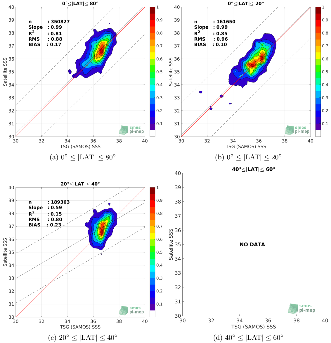
Figure 9: Contour maps of the concentration of SMOS SSS L2 v700 (ESA) SSS (y-axis) versus TSG (SAMOS) SSS (x-axis) at match-up pairs for different latitude bands. For each plot, the red line shows x=y . The black thin and dashed lines indicate a linear fit through the data cloud and the \pm 95\% confidence levels, respectively. The number match-up pairs n , the slope and R^2 coefficient of the linear fit, the root mean square (RMS) and the mean bias between satellite and in situ data are indicated for each latitude band in each plots.
