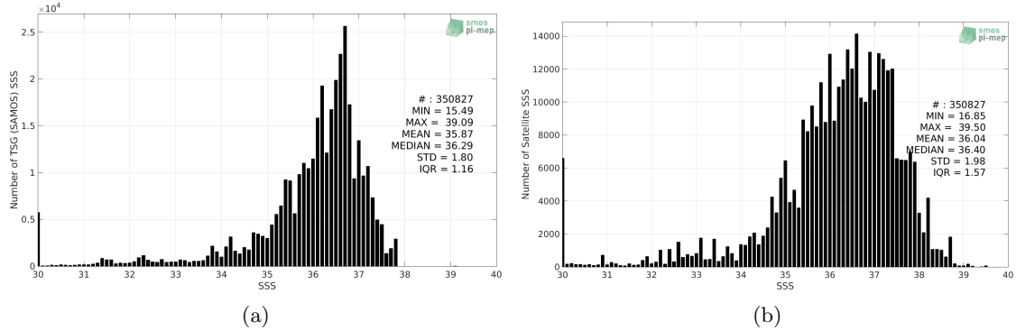
Figure 2: Histograms of SSS from TSG (SAMOS) (a) and SMOS SSS L2 v700 (ESA) (b) considering all match-up pairs per bins of 0.1 over the Amazon and Orinoco river plumes Pi-MEP region and for the full satellite product period.
