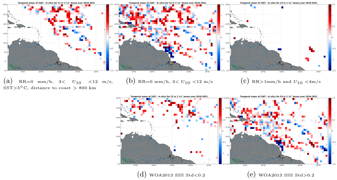
Figure 12: Temporal mean gridded over spatial boxes of size 1^\circ \times 1^\circ of \Delta SSS (SMOS SSS L2 v700 (ESA) - TSG (SAMOS)) for 5 different subdatasets corresponding to: RR=0 mm/h, 3 < U_{10} < 12 m/s, SST > 5^\circ\text{C} , distance to coast > 800 km (a), RR=0 mm/h, 3 < U_{10} < 12 m/s (b), RR > 1 mm/h and U_{10} < 4 m/s (c), WOA2013 SSS Std < 0.2 (d), WOA2013 SSS Std > 0.2 (e).
