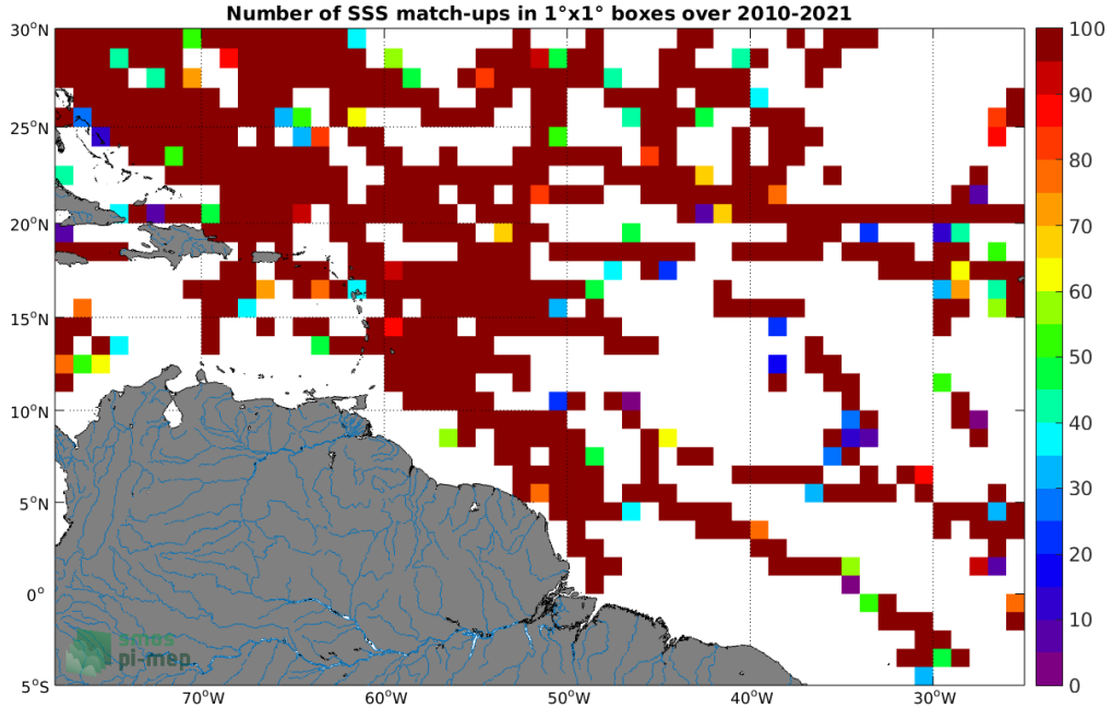
Figure 4: Number of SSS match-ups between TSG (SAMOS) SSS and the SMOS SSS L2 v700 (ESA) SSS product for the Amazon and Orinoco river plumes Pi-MEP region over 1^\circ \times 1^\circ boxes and for the full satellite product period.
