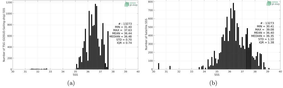
Figure 2: Histograms of SSS from TSG (GOSUD-Sailing-ship) (a) and SMOS SSS L2 v700 (ESA) (b) considering all match-up pairs per bins of 0.1 over the Amazon and Orinoco river plumes Pi-MEP region and for the full satellite product period.
