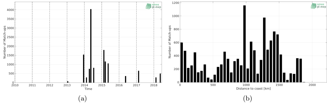
Figure 1: Number of match-ups between TSG (GOSUD-Sailing-ship) and SMOS SSS L2 v700 (ESA) SSS as a function of time (a) and as function of the distance to coast (b) over the Amazon and Orinoco river plumes Pi-MEP region and for the full satellite product period.
