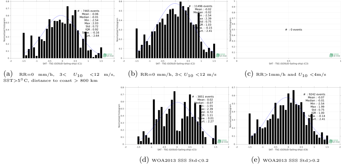
Figure 13: Normalized histogram of \Delta\text{SSS} (SMOS SSS L2 v700 (ESA) - TSG (GOSUD-Sailing-ship)) for 5 different subdatasets corresponding to: RR=0 mm/h, 3 < U_{10} < 12 m/s, SST > 5^\circ\text{C} , distance to coast > 800 km (a), RR=0 mm/h, 3 < U_{10} < 12 m/s (b), RR > 1\text{mm/h} and U_{10} < 4\text{m/s} (c), WOA2013 SSS Std < 0.2 (d), WOA2013 SSS Std > 0.2 (e).
