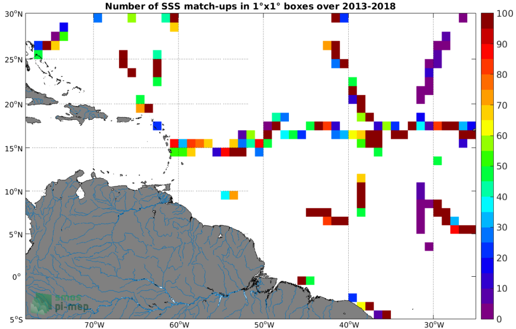
Figure 4: Number of SSS match-ups between TSG (GOSUD-Sailing-ship) SSS and the SMOS SSS L2 v700 (ESA) SSS product for the Amazon and Orinoco river plumes Pi-MEP region over 1^\circ \times 1^\circ boxes and for the full satellite product period.
