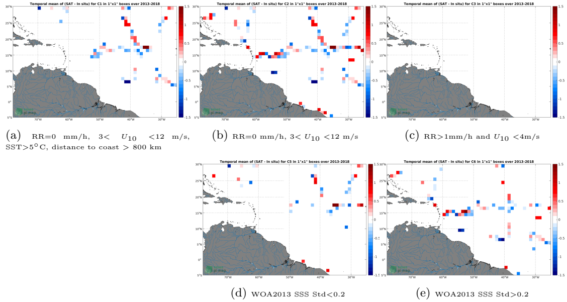
Figure 12: Temporal mean gridded over spatial boxes of size 1^\circ \times 1^\circ of \Delta SSS (SMOS SSS L2 v700 (ESA) - TSG (GOSUD-Sailing-ship)) for 5 different subdatasets corresponding to: RR=0 mm/h, 3 < U_{10} < 12 m/s, SST > 5^\circ C , distance to coast > 800 km (a), RR=0 mm/h, 3 < U_{10} < 12 m/s (b), RR > 1 mm/h and U_{10} < 4 m/s (c), WOA2013 SSS Std < 0.2 (d), WOA2013 SSS Std > 0.2 (e).
