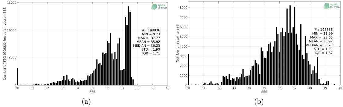
Figure 2: Histograms of SSS from TSG (GOSUD-Research-vessel) (a) and SMOS SSS L2 v700 (ESA) (b) considering all match-up pairs per bins of 0.1 over the Amazon and Orinoco river plumes Pi-MEP region and for the full satellite product period.
