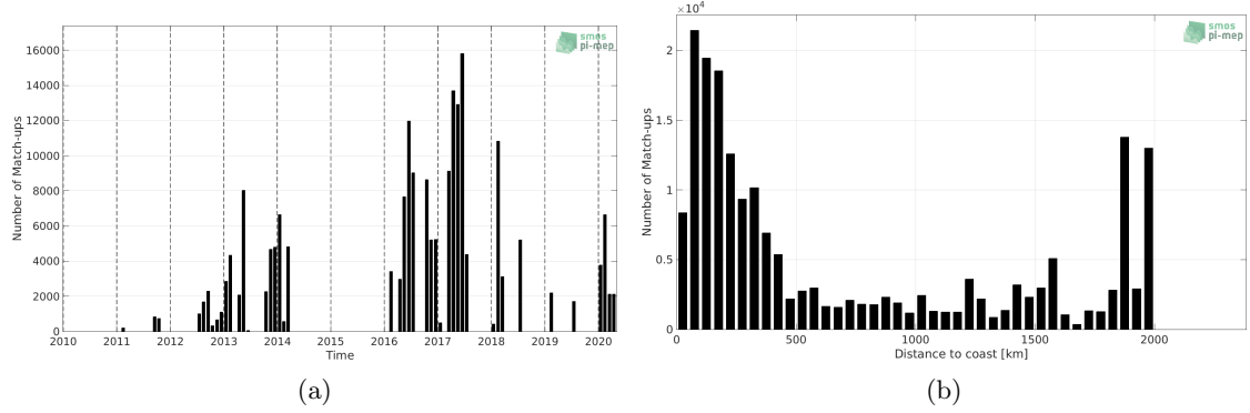
Figure 1: Number of match-ups between TSG (GOSUD-Research-vessel) and SMOS SSS L2 v700 (ESA) SSS as a function of time (a) and as function of the distance to coast (b) over the Amazon and Orinoco river plumes Pi-MEP region and for the full satellite product period.
