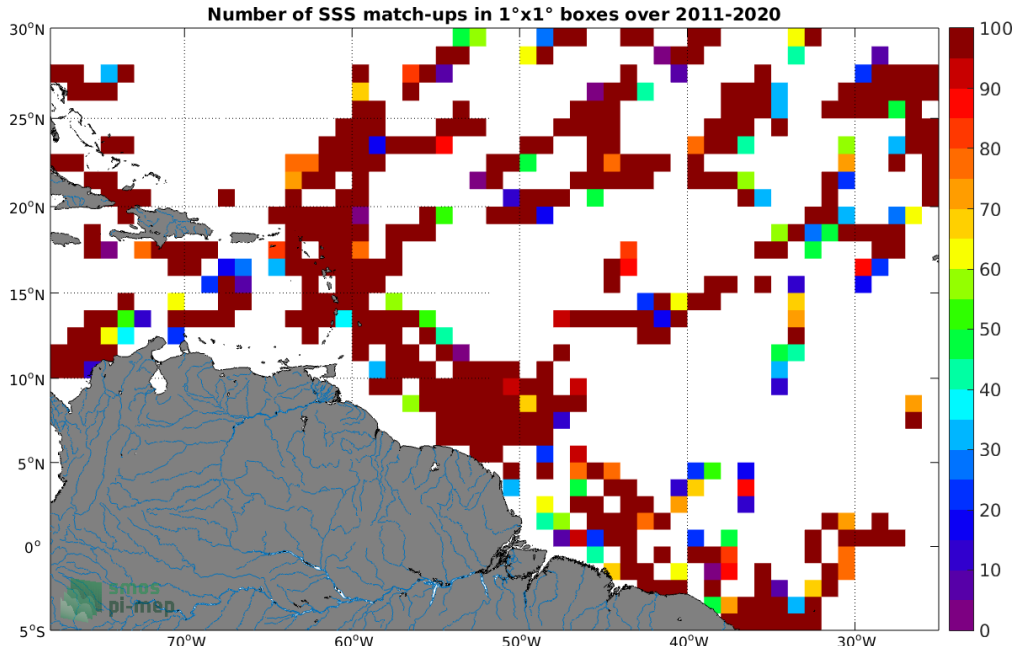
Figure 4: Number of SSS match-ups between TSG (GOSUD-Research-vessel) SSS and the SMOS SSS L2 v700 (ESA) SSS product for the Amazon and Orinoco river plumes Pi-MEP region over 1^\circ \times 1^\circ boxes and for the full satellite product period.
