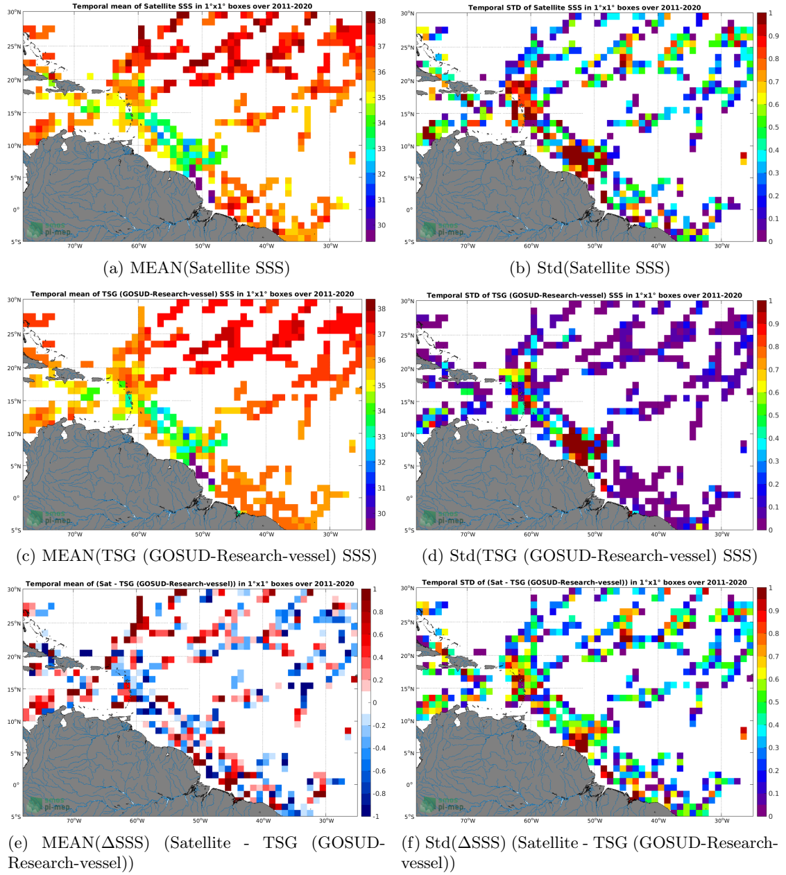
Figure 6: Temporal mean (left) and Std (right) of SSS from SMOS SSS L2 v700 (ESA) (top), TSG (GOSUD-Research-vessel) (middle), and of \Delta SSS (Satellite - TSG (GOSUD-Research-vessel)). Only match-up pairs are used to generate these maps.
