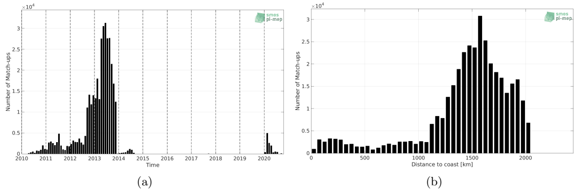
Figure 1: Number of match-ups between Surface drifters and SMOS SSS L2 v700 (ESA) SSS as a function of time (a) and as function of the distance to coast (b) over the Amazon and Orinoco river plumes Pi-MEP region and for the full satellite product period.
