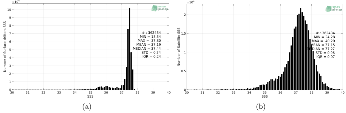
Figure 2: Histograms of SSS from Surface drifters (a) and SMOS SSS L2 v700 (ESA) (b) considering all match-up pairs per bins of 0.1 over the Amazon and Orinoco river plumes Pi-MEP region and for the full satellite product period.
