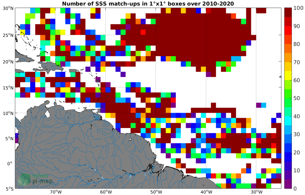
Figure 3: Number of SSS match-ups between Surface drifters SSS and the SMOS SSS L2 v700 (ESA) SSS product for the Amazon and Orinoco river plumes Pi-MEP region over 1^\circ \times 1^\circ boxes and for the full satellite product period.
