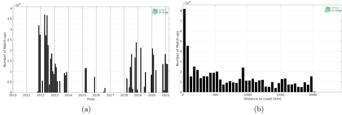
Figure 1: Number of match-ups between TSG (SAMOS) and SMAP SSS L4 OI v1 - 7 Days (IPRC) SSS as a function of time (a) and as function of the distance to coast (b) over the Amazon and Orinoco river plumes Pi-MEP region and for the full satellite product period.
