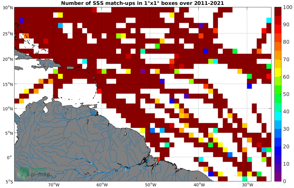
Figure 4: Number of SSS match-ups between TSG (SAMOS) SSS and the SMAP SSS L4 OI v1 - 7 Days (IPRC) SSS product for the Amazon and Orinoco river plumes Pi-MEP region over 1^\circ \times 1^\circ boxes and for the full satellite product period.
