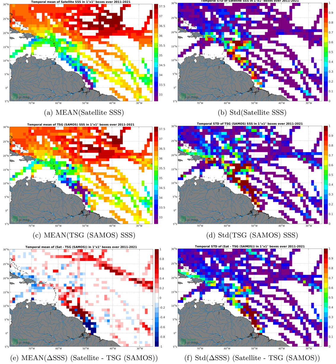
Figure 6: Temporal mean (left) and Std (right) of SSS from SMAP SSS L4 OI v1 - 7 Days (IPRC) (top), TSG (SAMOS) (middle), and of \Delta SSS (Satellite - TSG (SAMOS)). Only match-up pairs are used to generate these maps.
