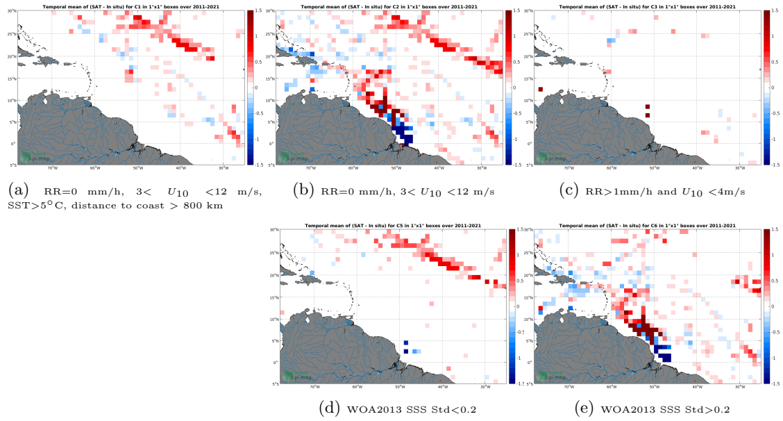
Figure 12: Temporal mean gridded over spatial boxes of size 1^\circ \times 1^\circ of \Delta SSS (SMAP SSS L4 OI v1 - 7 Days (IPRC) - TSG (SAMOS)) for 5 different subdatasets corresponding to: RR=0 mm/h, 3 < U_{10} < 12 m/s, SST > 5^\circ C , distance to coast > 800 km (a), RR=0 mm/h, 3 < U_{10} < 12 m/s (b), RR > 1 mm/h and U_{10} < 4 m/s (c), WOA2013 SSS Std < 0.2 (d), WOA2013 SSS Std > 0.2 (e).
