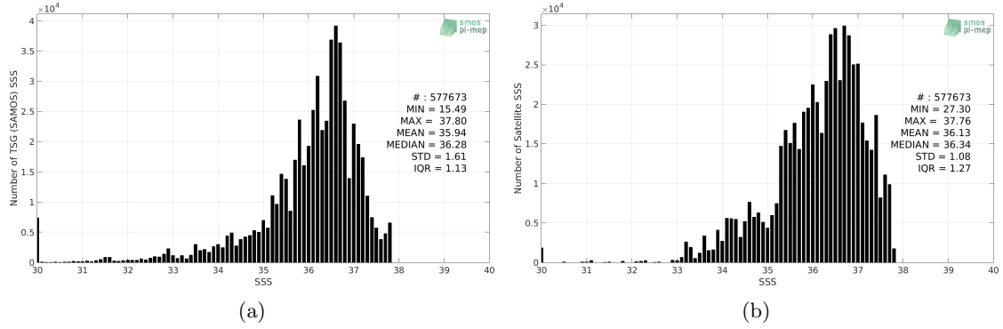
Figure 2: Histograms of SSS from TSG (SAMOS) (a) and SMAP SSS L4 OI v1 - 7 Days (IPRC) (b) considering all match-up pairs per bins of 0.1 over the Amazon and Orinoco river plumes Pi-MEP region and for the full satellite product period.
