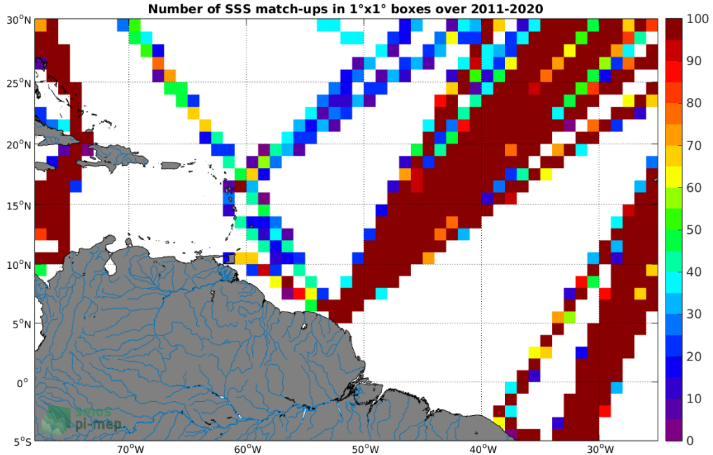
Figure 4: Number of SSS match-ups between TSG (LEGOS-DM) SSS and the SMAP SSS L4 OI v1 - 7 Days (IPRC) SSS product for the Amazon and Orinoco river plumes Pi-MEP region over 1^\circ \times 1^\circ boxes and for the full satellite product period.
