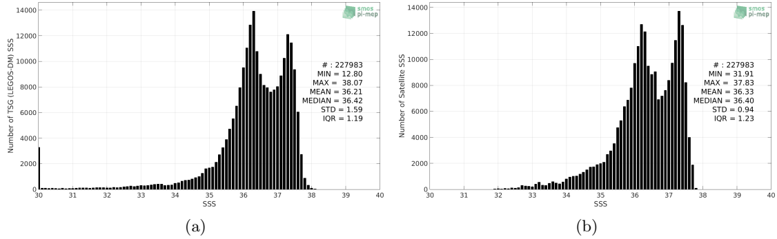
Figure 2: Histograms of SSS from TSG (LEGOS-DM) (a) and SMAP SSS L4 OI v1 - 7 Days (IPRC) (b) considering all match-up pairs per bins of 0.1 over the Amazon and Orinoco river plumes Pi-MEP region and for the full satellite product period.
