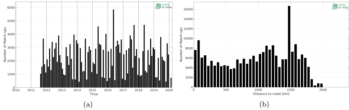
Figure 1: Number of match-ups between TSG (LEGOS-DM) and SMAP SSS L4 OI v1 - 7 Days (IPRC) SSS as a function of time (a) and as function of the distance to coast (b) over the Amazon and Orinoco river plumes Pi-MEP region and for the full satellite product period.
