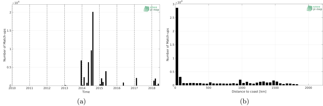
Figure 1: Number of match-ups between TSG (GOSUD-Sailing-ship) and SMAP SSS L4 OI v1 - 7 Days (IPRC) SSS as a function of time (a) and as function of the distance to coast (b) over the Amazon and Orinoco river plumes Pi-MEP region and for the full satellite product period.
