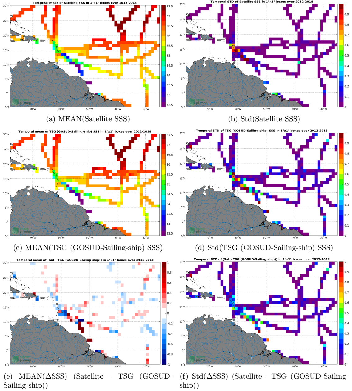
Figure 6: Temporal mean (left) and Std (right) of SSS from SMAP SSS L4 OI v1 - 7 Days (IPRC) (top), TSG (GOSUD-Sailing-ship) (middle), and of \Delta SSS (Satellite - TSG (GOSUD-Sailing-ship)). Only match-up pairs are used to generate these maps.
