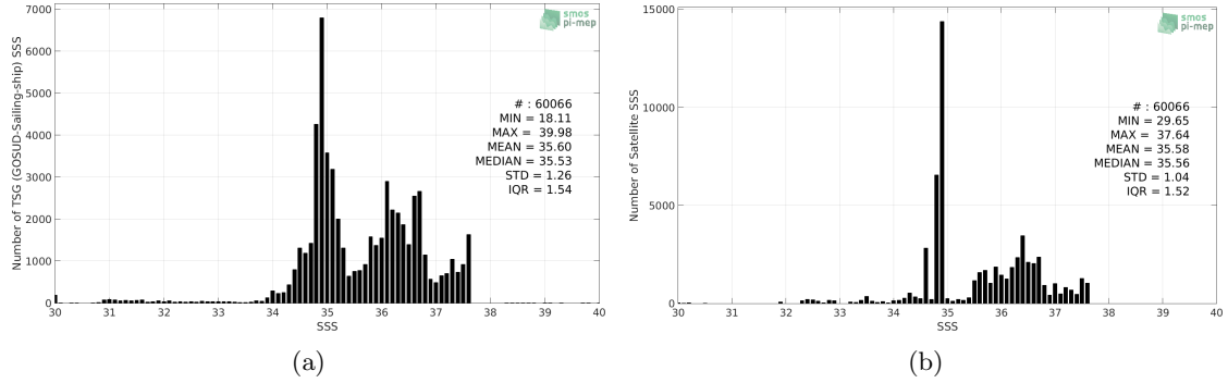
Figure 2: Histograms of SSS from TSG (GOSUD-Sailing-ship) (a) and SMAP SSS L4 OI v1 - 7 Days (IPRC) (b) considering all match-up pairs per bins of 0.1 over the Amazon and Orinoco river plumes Pi-MEP region and for the full satellite product period.
