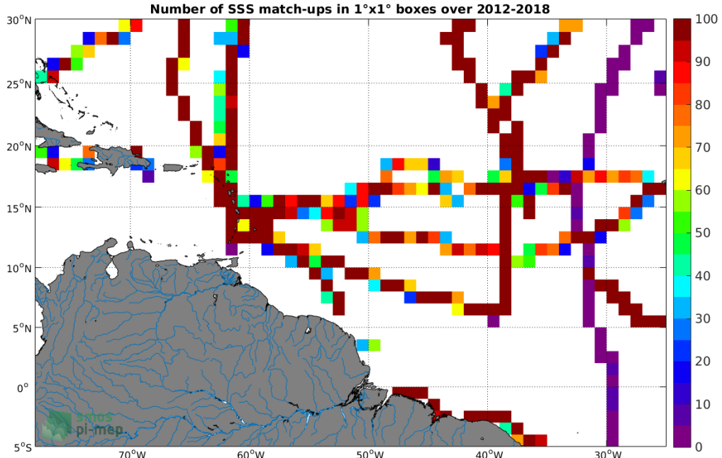
Figure 4: Number of SSS match-ups between TSG (GOSUD-Sailing-ship) SSS and the SMAP SSS L4 OI v1 - 7 Days (IPRC) SSS product for the Amazon and Orinoco river plumes Pi-MEP region over 1^\circ \times 1^\circ boxes and for the full satellite product period.
