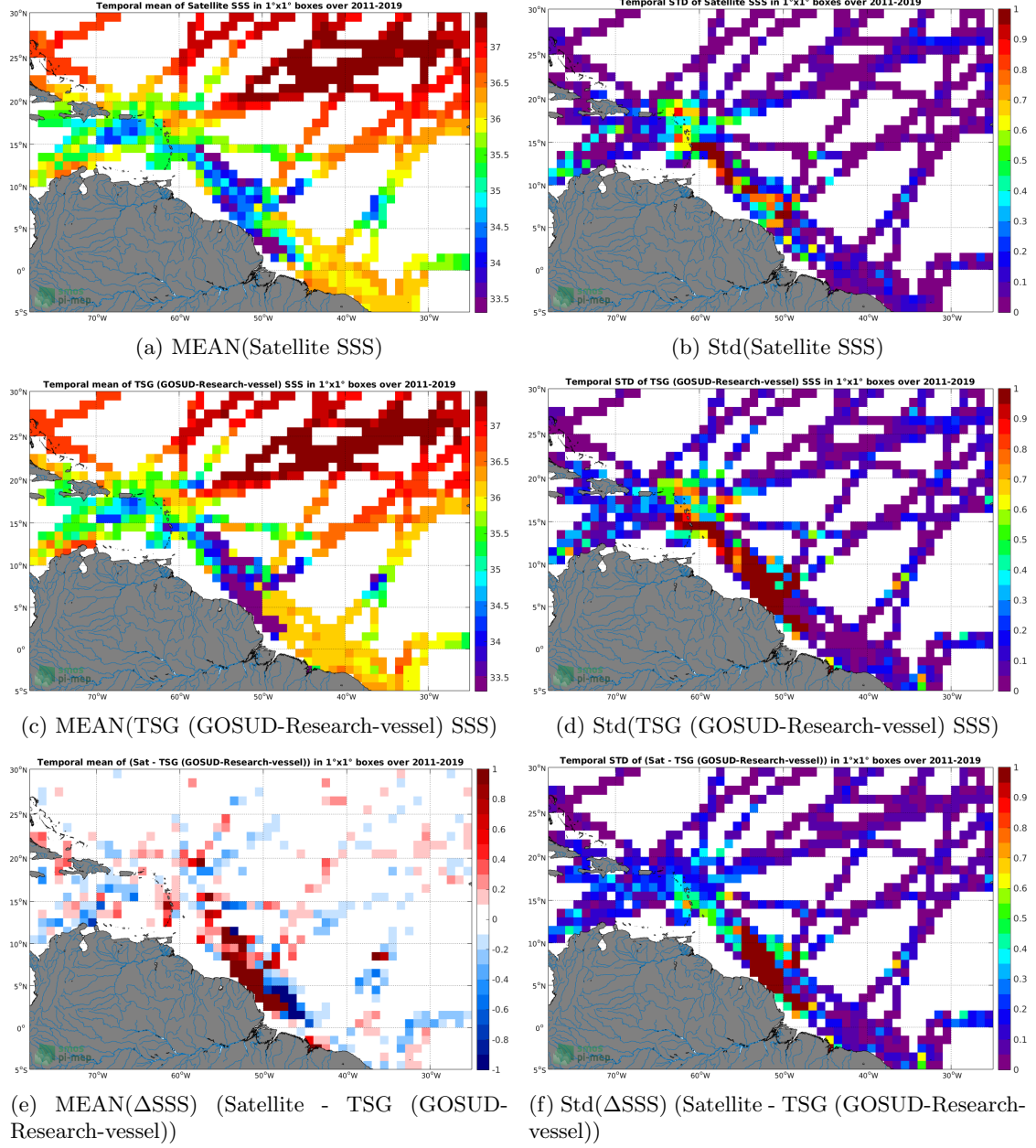
Figure 6: Temporal mean (left) and Std (right) of SSS from SMAP SSS L4 OI v1 - 7day (IPRC) (top), TSG (GOSUD-Research-vessel) (middle), and of \Delta SSS (Satellite - TSG (GOSUD-Research-vessel)). Only match-up pairs are used to generate these maps.
