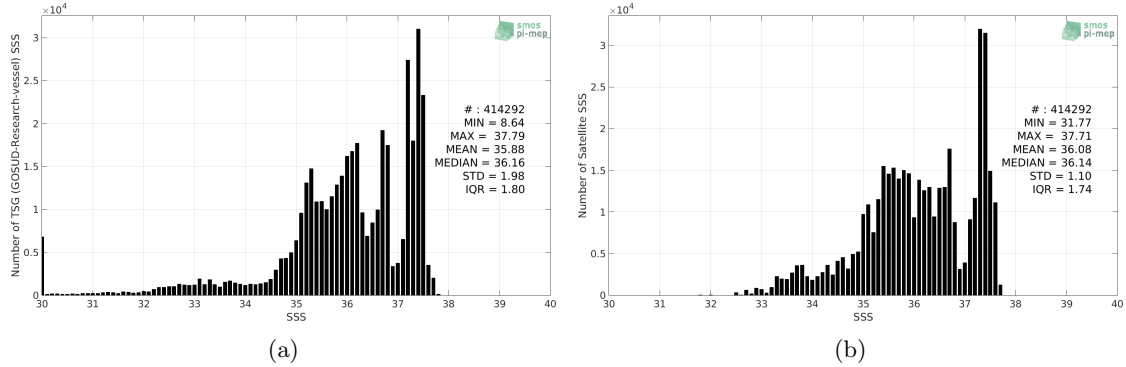
Figure 2: Histograms of SSS from TSG (GOSUD-Research-vessel) (a) and SMAP SSS L4 OI v1 - 7day (IPRC) (b) considering all match-up pairs per bins of 0.1 over the Amazon and Orinoco river plumes Pi-MEP region and for the full satellite product period.
