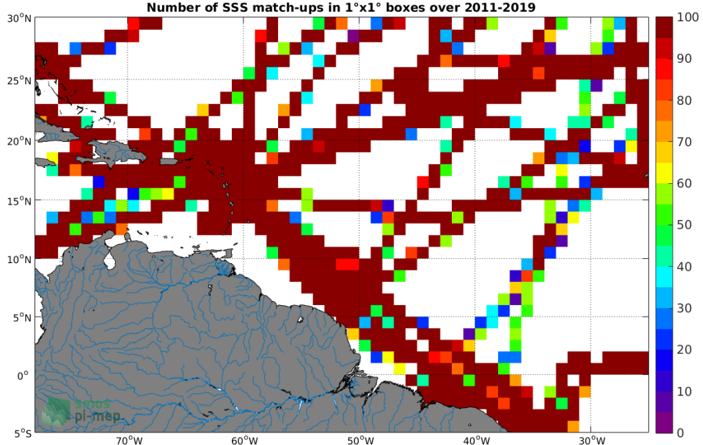
Figure 4: Number of SSS match-ups between TSG (GOSUD-Research-vessel) SSS and the SMAP SSS L4 OI v1 - 7day (IPRC) SSS product for the Amazon and Orinoco river plumes Pi-MEP region over 1^\circ \times 1^\circ boxes and for the full satellite product period.
