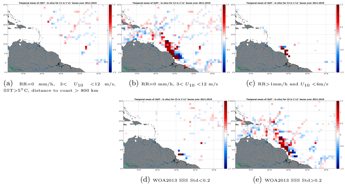
Figure 12: Temporal mean gridded over spatial boxes of size 1^\circ \times 1^\circ of \Delta SSS (SMAP SSS L4 OI v1 - 7day (IPRC) - TSG (GOSUD-Research-vessel)) for 5 different subdatasets corresponding to: RR=0 mm/h, 3 < U_{10} < 12 m/s, SST >5^\circ C, distance to coast > 800 km (a), RR=0 mm/h, 3 < U_{10} < 12 m/s (b), RR >1 mm/h and U_{10} < 4 m/s (c), WOA2013 SSS Std <0.2 (d), WOA2013 SSS Std >0.2 (e).
