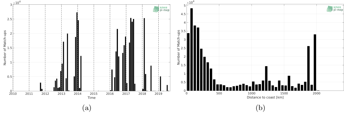
Figure 1: Number of match-ups between TSG (GOSUD-Research-vessel) and SMAP SSS L4 OI v1 - 7day (IPRC) SSS as a function of time (a) and as function of the distance to coast (b) over the Amazon and Orinoco river plumes Pi-MEP region and for the full satellite product period.
