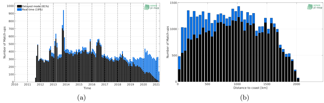
Figure 1: Number of match-ups between Argo and SMAP SSS L4 OI v1 - 7 Days (IPRC) SSS as a function of time (a) and as function of the distance to coast (b) over the Amazon and Orinoco river plumes Pi-MEP region and for the full satellite product period.
