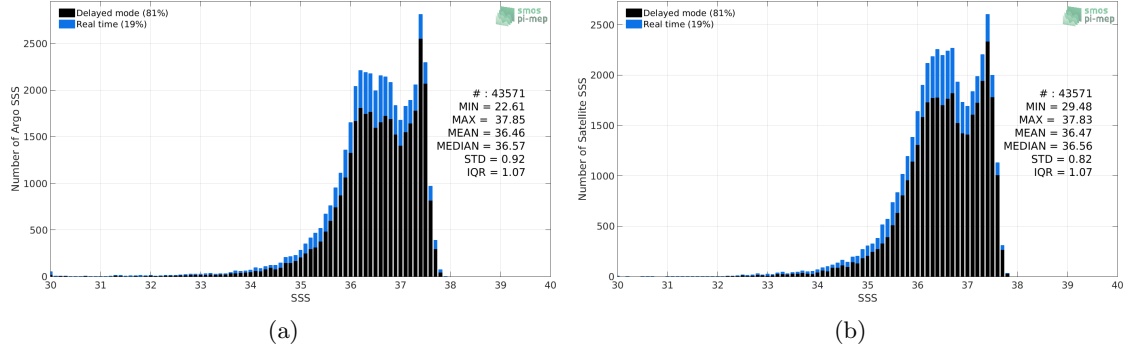
Figure 2: Histograms of SSS from Argo (a) and SMAP SSS L4 OI v1 - 7 Days (IPRC) (b) considering all match-up pairs per bins of 0.1 over the Amazon and Orinoco river plumes Pi-MEP region and for the full satellite product period.
