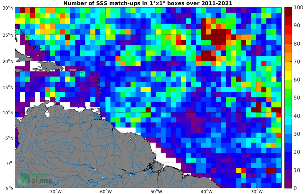
Figure 4: Number of SSS match-ups between Argo SSS and the SMAP SSS L4 OI v1 - 7 Days (IPRC) SSS product for the Amazon and Orinoco river plumes Pi-MEP region over 1^\circ \times 1^\circ boxes and for the full satellite product period.
