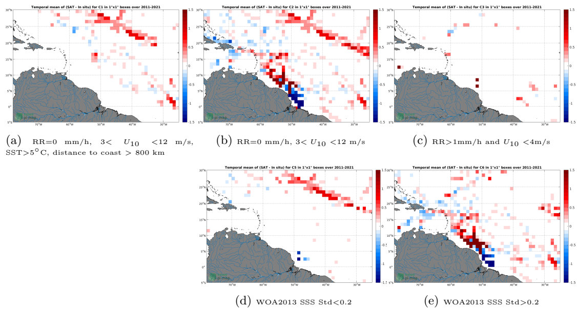
Figure 12: Temporal mean gridded over spatial boxes of size 1^\circ \times 1^\circ of \Delta SSS (SMAP SSS L4 OI v1 - Monthly (IPRC) - TSG (SAMOS)) for 5 different subdatasets corresponding to: RR=0 mm/h, 3 < U_{10} < 12 m/s, SST > 5^\circ C , distance to coast > 800 km (a), RR=0 mm/h, 3 < U_{10} < 12 m/s (b), RR > 1 mm/h and U_{10} < 4 m/s (c), WOA2013 SSS Std < 0.2 (d), WOA2013 SSS Std > 0.2 (e).
