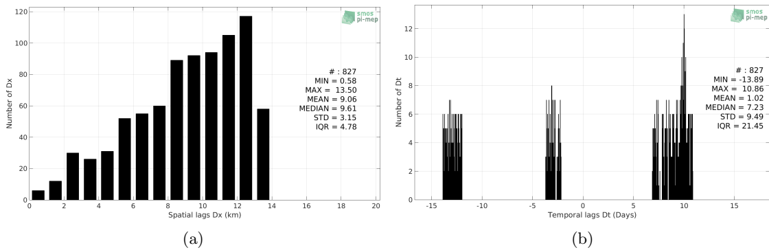
Figure 5: Histograms of the spatial (a) and temporal (b) lags between the location/time of the TSG (Polarstern) measurement and the date of the corresponding SMAP SSS L4 OI v1 - Monthly (IPRC) SSS pixel.
