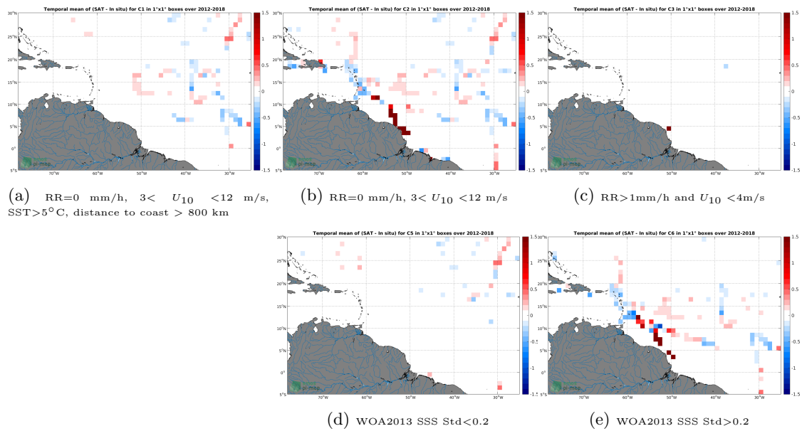
Figure 12: Temporal mean gridded over spatial boxes of size 1^\circ \times 1^\circ of \Delta\text{SSS} (SMAP SSS L4 OI v1 - Monthly (IPRC) - TSG (GOSUD-Sailing-ship)) for 5 different subdatasets corresponding to:RR=0 mm/h, 3 < U_{10} < 12 m/s, SST>5°C, distance to coast > 800 km (a), RR=0 mm/h, 3 < U_{10} < 12 m/s (b), RR>1mm/h and U_{10} < 4 m/s (c), WOA2013 SSS Std<0.2 (d), WOA2013 SSS Std>0.2 (e).
