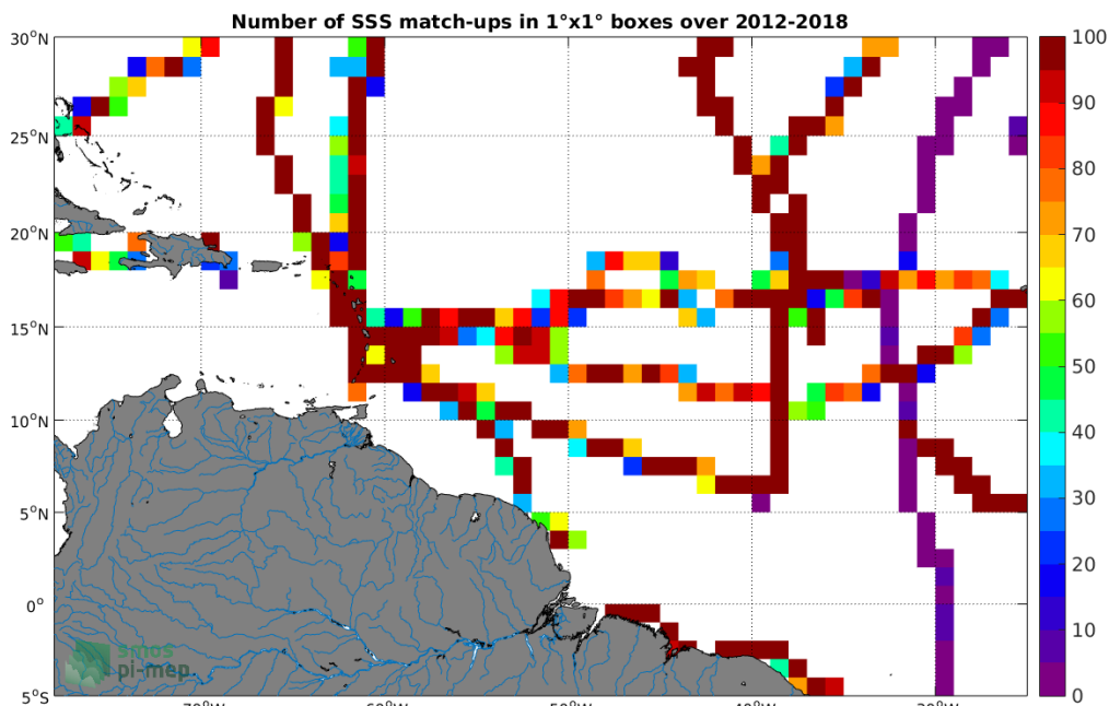
Figure 4: Number of SSS match-ups between TSG (GOSUD-Sailing-ship) SSS and the SMAP SSS L4 OI v1 - Monthly (IPRC) SSS product for the Amazon and Orinoco river plumes Pi-MEP region over 1°x1° boxes and for the full satellite product period.
