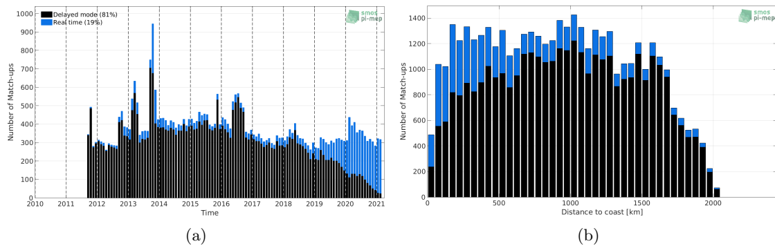
Figure 1: Number of match-ups between Argo and SMAP SSS L4 OI v1 - Monthly (IPRC) SSS as a function of time (a) and as function of the distance to coast (b) over the Amazon and Orinoco river plumes Pi-MEP region and for the full satellite product period.
