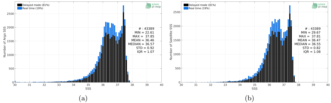
Figure 2: Histograms of SSS from Argo (a) and SMAP SSS L4 OI v1 - Monthly (IPRC) (b) considering all match-up pairs per bins of 0.1 over the Amazon and Orinoco river plumes Pi-MEP region and for the full satellite product period.
