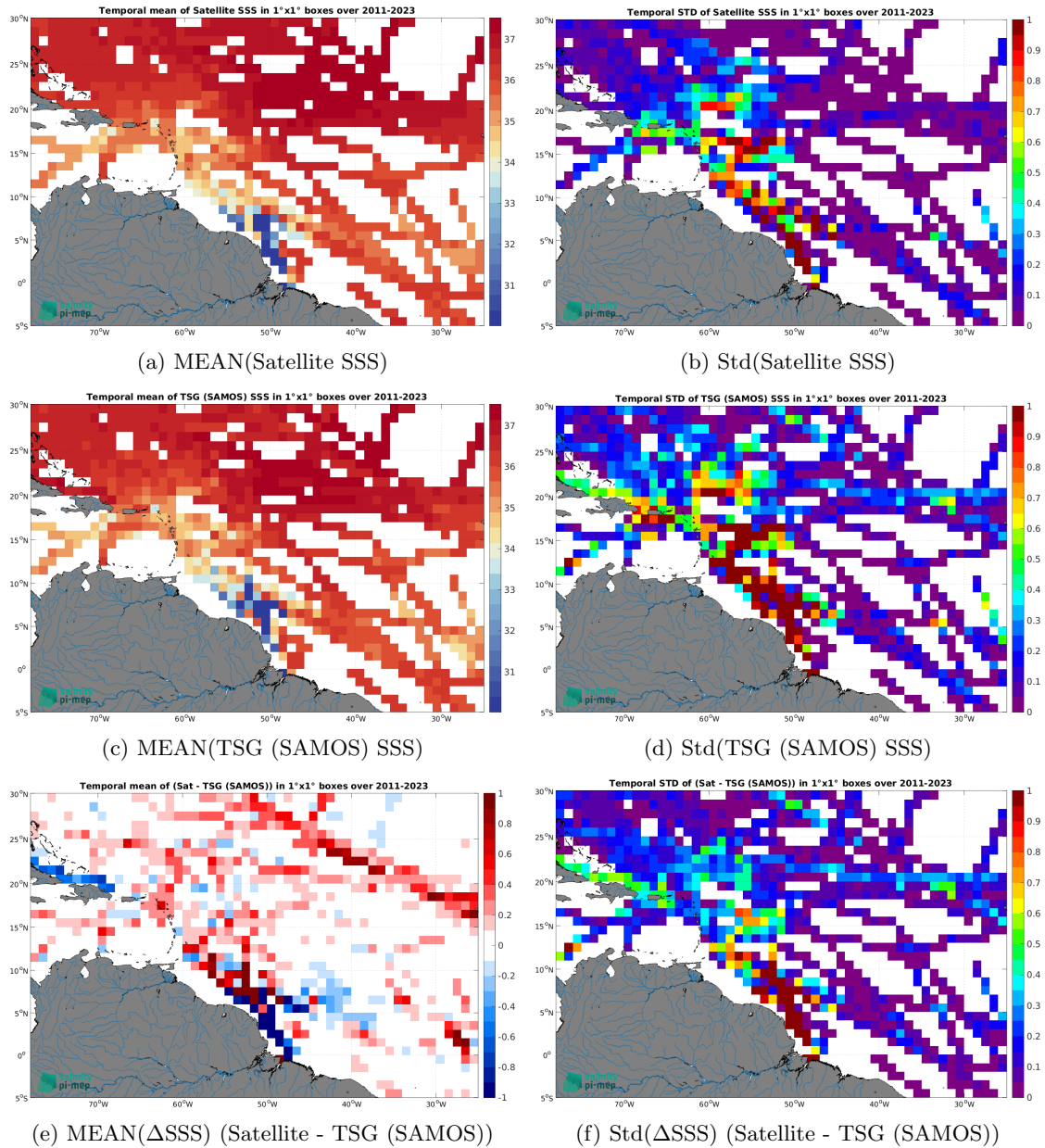
Figure 7: Temporal mean (left) and Std (right) of SSS from SMAP SSS L4 OI v3 - Monthly (ESR) (top), TSG (SAMOS) (middle), and of \Delta SSS (Satellite - TSG (SAMOS)). Only match-up pairs are used to generate these maps.
