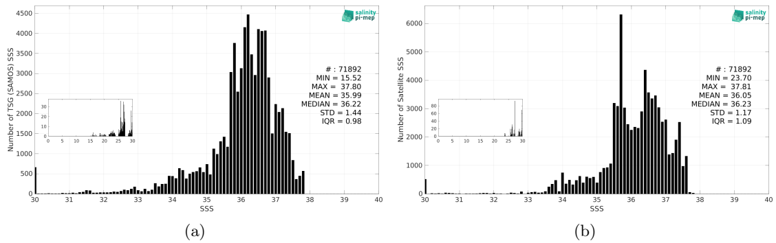
Figure 3: Histograms of SSS from TSG (SAMOS) (a) and SMAP SSS L4 OI v3 - Monthly (ESR) (b) considering all match-up pairs per bins of 0.1 over the Amazon and Orinoco river plumes Pi-MEP region and for the full satellite product period.
