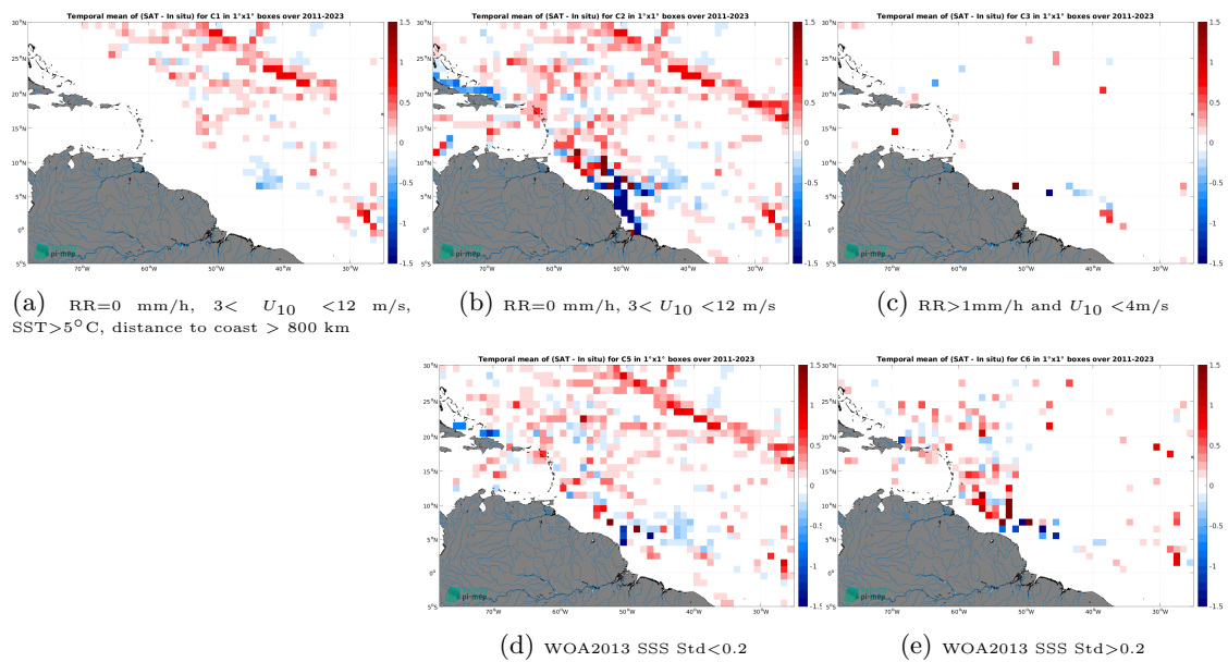
Figure 14: Temporal mean gridded over spatial boxes of size 1^\circ \times 1^\circ of \Delta SSS (SMAP SSS L4 OI v3 - Monthly (ESR) - TSG (SAMOS)) for 5 different subdatasets corresponding to:RR=0 mm/h, 3 < U_{10} < 12 m/s, SST >5^\circ\text{C} , distance to coast > 800 km (a), RR=0 mm/h, 3 < U_{10} < 12 m/s (b), RR >1 mm/h and U_{10} < 4 m/s (c), WOA2013 SSS Std <0.2 (d), WOA2013 SSS Std >0.2 (e).
