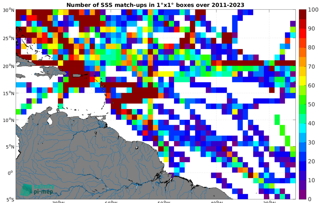
Figure 5: Number of SSS match-ups between TSG (SAMOS) SSS and the SMAP SSS L4 OI v3 - Monthly (ESR) SSS product for the Amazon and Orinoco river plumes Pi-MEP region over 1^\circ \times 1^\circ boxes and for the full satellite product period.
