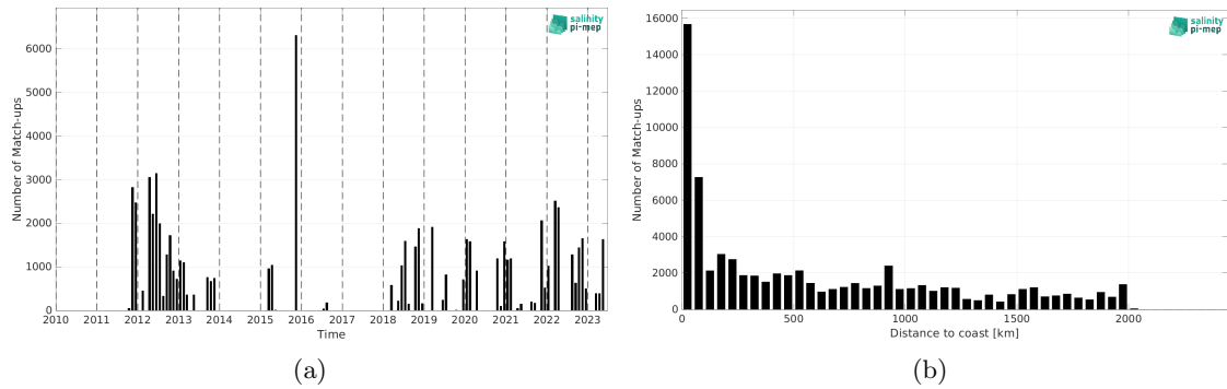
Figure 2: Number of match-ups between TSG (SAMOS) and SMAP SSS L4 OI v3 - Monthly (ESR) SSS as a function of time (a) and as function of the distance to coast (b) over the Amazon and Orinoco river plumes Pi-MEP region and for the full satellite product period.
