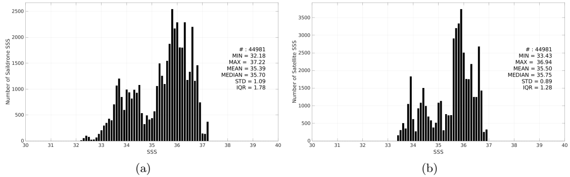
Figure 3: Histograms of SSS from Saildrone (a) and SMAP SSS L4 OI v3 - Monthly (ESR) (b) considering all match-up pairs per bins of 0.1 over the Amazon and Orinoco river plumes Pi-MEP region and for the full satellite product period.
