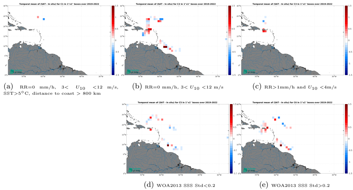
Figure 14: Temporal mean gridded over spatial boxes of size 1^\circ \times 1^\circ of \Delta SSS (SMAP SSS L4 OI v3 - Monthly (ESR) - Saldrone) for 5 different subdatasets corresponding to:RR=0 mm/h, 3 < U_{10} < 12 m/s, SST >5^\circ\text{C} , distance to coast > 800 km (a), RR=0 mm/h, 3 < U_{10} < 12 m/s (b), RR >1 mm/h and U_{10} < 4 m/s (c), WOA2013 SSS Std <0.2 (d), WOA2013 SSS Std >0.2 (e).
