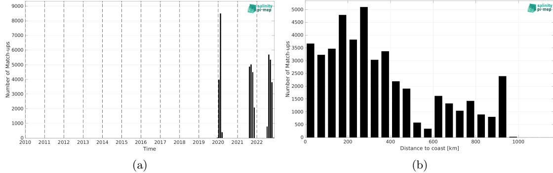
Figure 2: Number of match-ups between Saildrone and SMAP SSS L4 OI v3 - Monthly (ESR) SSS as a function of time (a) and as function of the distance to coast (b) over the Amazon and Orinoco river plumes Pi-MEP region and for the full satellite product period.
