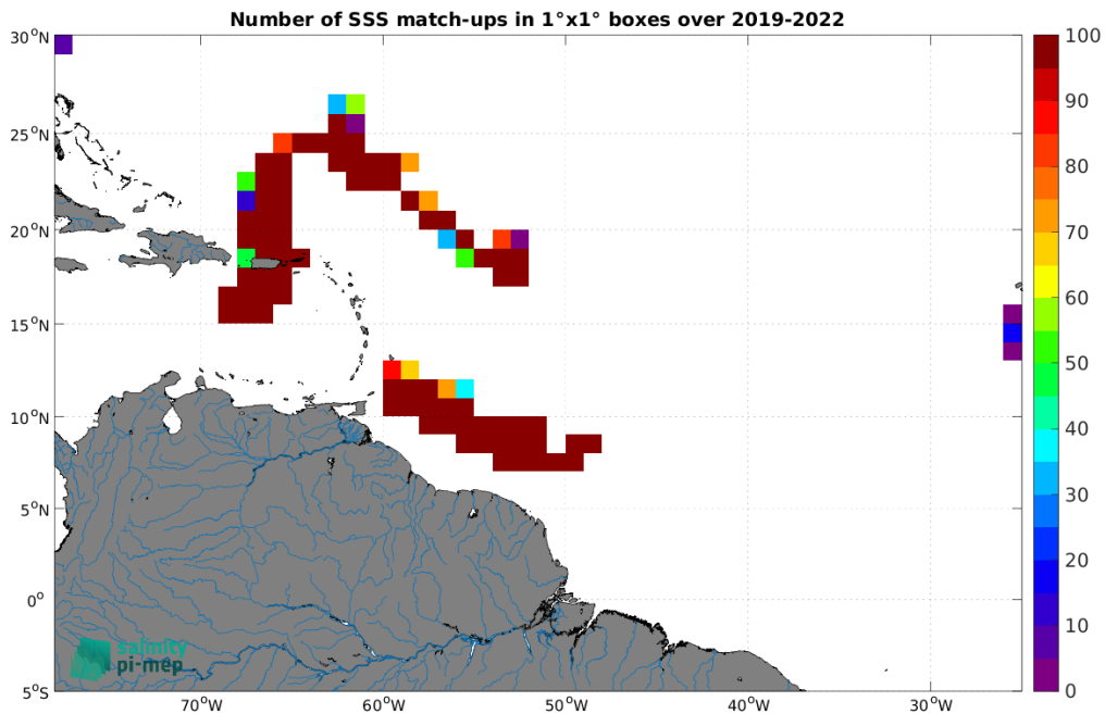
Figure 5: Number of SSS match-ups between Sailability SSS and the SMAP SSS L4 OI v3 - Monthly (ESR) SSS product for the Amazon and Orinoco river plumes Pi-MEP region over 1^\circ \times 1^\circ boxes and for the full satellite product period.
