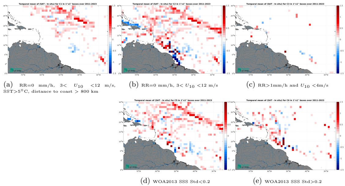
Figure 14: Temporal mean gridded over spatial boxes of size 1^\circ \times 1^\circ of \Delta SSS (SMAP SSS L4 OI v3 - Daily (ESR) - TSG (SAMOS)) for 5 different subdatasets corresponding to: RR=0 mm/h, 3 < U_{10} < 12 m/s, SST > 5^\circ C , distance to coast > 800 km (a), RR=0 mm/h, 3 < U_{10} < 12 m/s (b), RR > 1 mm/h and U_{10} < 4 m/s (c), WOA2013 SSS Std < 0.2 (d), WOA2013 SSS Std > 0.2 (e).
