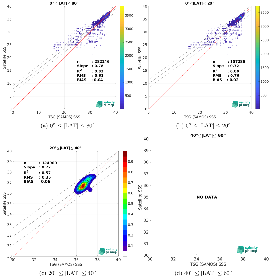
Figure 10: Contour maps of the concentration of SMAP SSS L4 OI v3 - Daily (ESR) SSS (y-axis) versus TSG (SAMOS) SSS (x-axis) at match-up pairs for different latitude bands. For each plot, the red line shows x=y . The black thin and dashed lines indicate a linear fit through the data cloud and the \pm 95\% confidence levels, respectively. The number match-up pairs n , the slope and R^2 coefficient of the linear fit, the root mean square (RMS) and the mean bias between satellite and in situ data are indicated for each latitude band in each plots.
