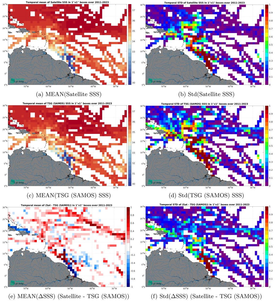
Figure 7: Temporal mean (left) and Std (right) of SSS from SMAP SSS L4 OI v3 - Daily (ESR) (top), TSG (SAMOS) (middle), and of \Delta SSS (Satellite - TSG (SAMOS)). Only match-up pairs are used to generate these maps.
