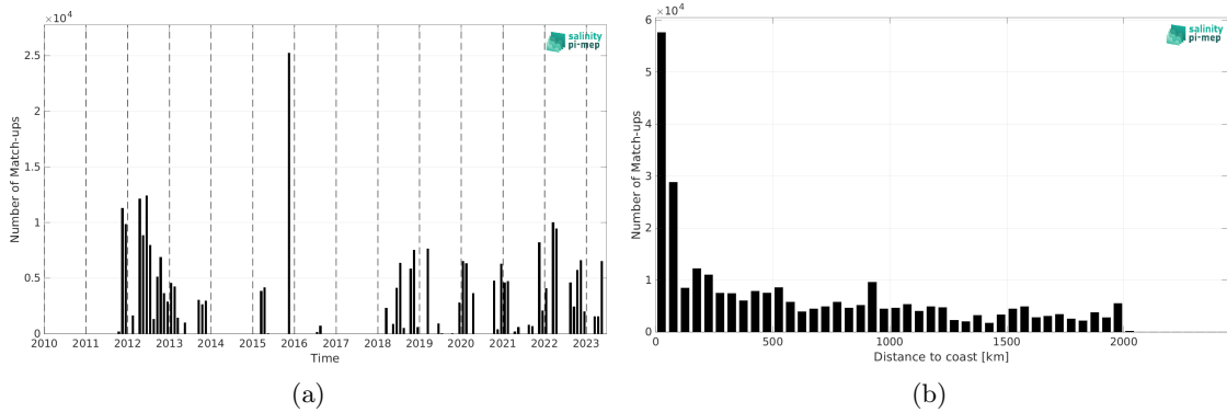
Figure 2: Number of match-ups between TSG (SAMOS) and SMAP SSS L4 OI v3 - Daily (ESR) SSS as a function of time (a) and as function of the distance to coast (b) over the Amazon and Orinoco river plumes Pi-MEP region and for the full satellite product period.
