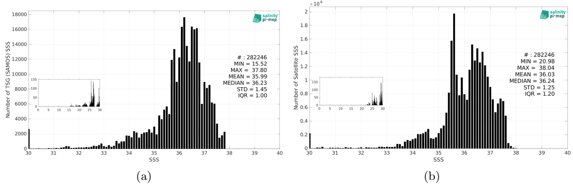
Figure 3: Histograms of SSS from TSG (SAMOS) (a) and SMAP SSS L4 OI v3 - Daily (ESR) (b) considering all match-up pairs per bins of 0.1 over the Amazon and Orinoco river plumes Pi-MEP region and for the full satellite product period.
