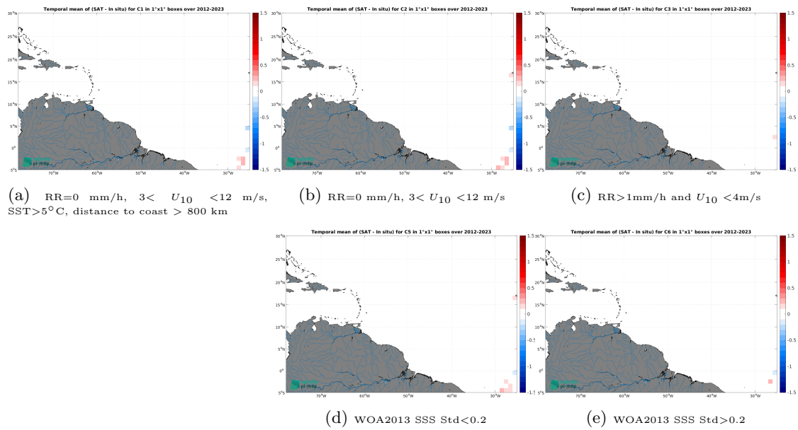
Figure 14: Temporal mean gridded over spatial boxes of size 1^\circ \times 1^\circ of \Delta SSS (SMAP SSS L4 OI v3 - Daily (ESR) - TSG (Polarstern)) for 5 different subdatasets corresponding to: RR=0 mm/h, 3 < U_{10} < 12 m/s, SST > 5^\circ C , distance to coast > 800 km (a), RR=0 mm/h, 3 < U_{10} < 12 m/s (b), RR > 1 mm/h and U_{10} < 4 m/s (c), WOA2013 SSS Std < 0.2 (d), WOA2013 SSS Std > 0.2 (e).
