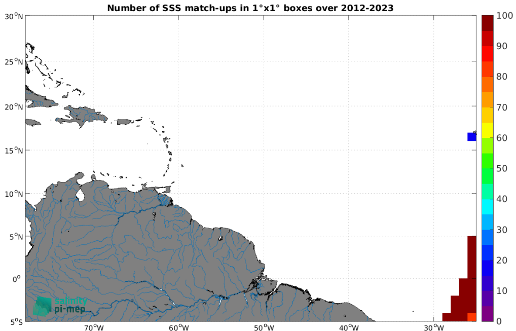
Figure 5: Number of SSS match-ups between TSG (Polarstern) SSS and the SMAP SSS L4 OI v3 - Daily (ESR) SSS product for the Amazon and Orinoco river plumes Pi-MEP region over 1^\circ \times 1^\circ boxes and for the full satellite product period.
