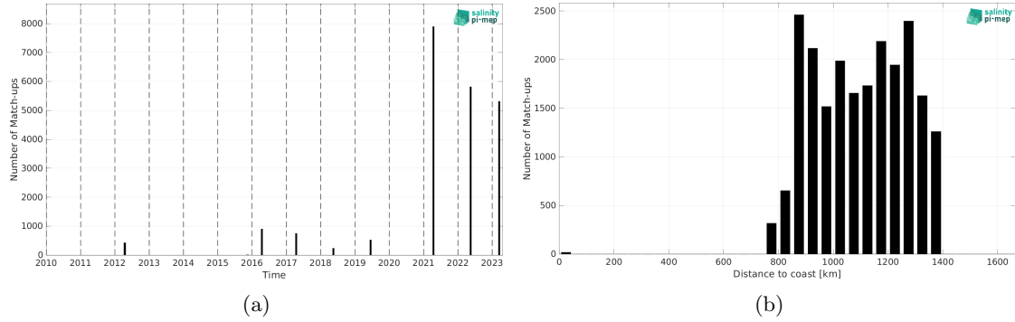
Figure 2: Number of match-ups between TSG (Polarstern) and SMAP SSS L4 OI v3 - Daily (ESR) SSS as a function of time (a) and as function of the distance to coast (b) over the Amazon and Orinoco river plumes Pi-MEP region and for the full satellite product period.
