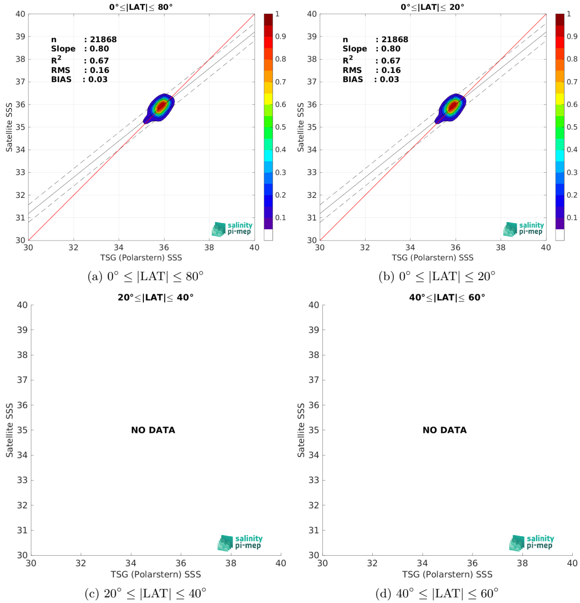
Figure 10: Contour maps of the concentration of SMAP SSS L4 OI v3 - Daily (ESR) SSS (y-axis) versus TSG (Polarstern) SSS (x-axis) at match-up pairs for different latitude bands. For each plot, the red line shows x=y . The black thin and dashed lines indicate a linear fit through the data cloud and the \pm 95\% confidence levels, respectively. The number match-up pairs n , the slope and R^2 coefficient of the linear fit, the root mean square (RMS) and the mean bias between satellite and in situ data are indicated for each latitude band in each plots.
