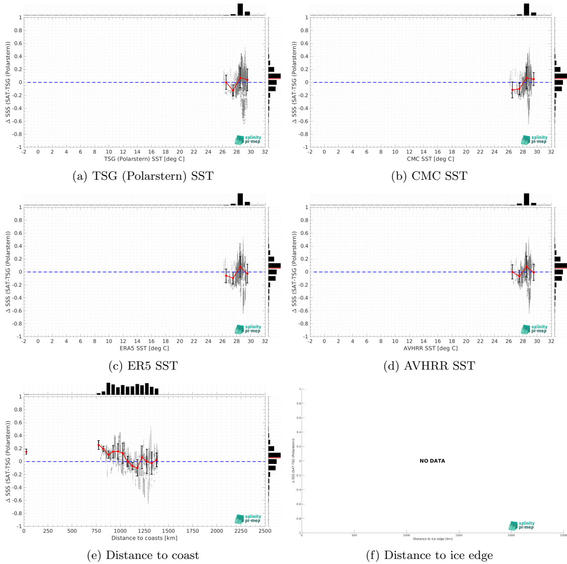
Figure 13: \Delta\text{SSS} (Satellite - TSG (Polarstern)) sorted as function of TSG (Polarstern) SST values (a), CMC SST (b), ERA5 SST (c), AVHRR SST (d), distance to coast (e) and distance to ice edge (f). In all plots the median and Std of \Delta\text{SSS} for each bin is indicated by the red curves and black vertical thick bars ( \pm 1 Std). Links to similar figures sorted as function of Sea ice fraction and in situ measurement depth .
