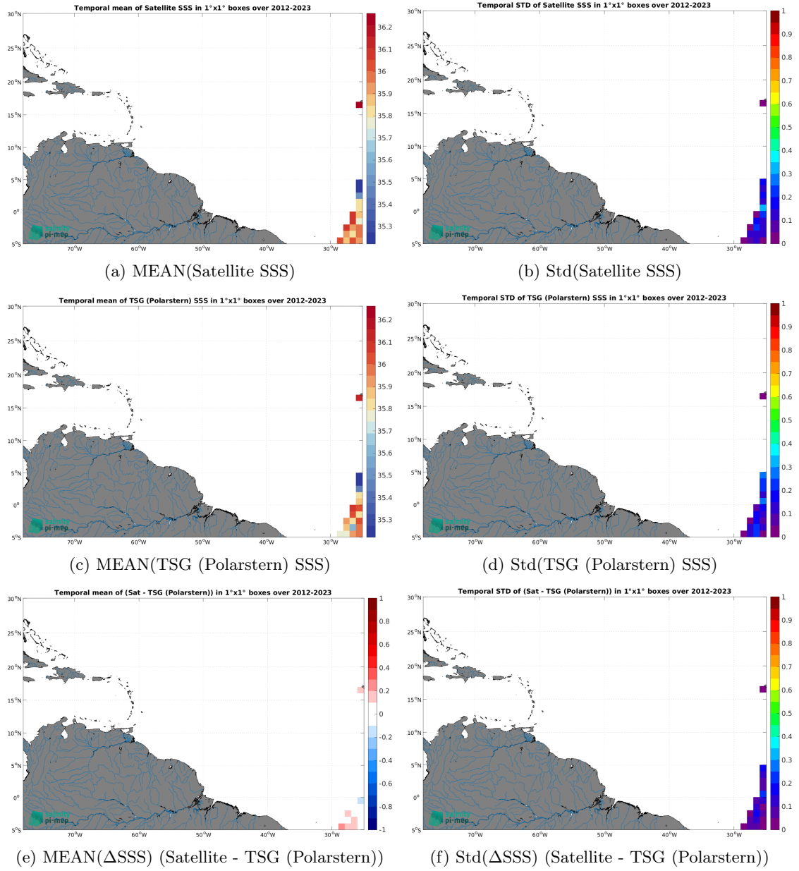
Figure 7: Temporal mean (left) and Std (right) of SSS from SMAP SSS L4 OI v3 - Daily (ESR) (top), TSG (Polarstern) (middle), and of \Delta SSS (Satellite - TSG (Polarstern)). Only match-up pairs are used to generate these maps.
