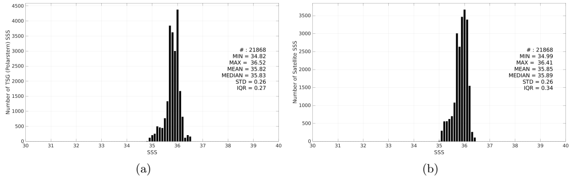
Figure 3: Histograms of SSS from TSG (Polarstern) (a) and SMAP SSS L4 OI v3 - Daily (ESR) (b) considering all match-up pairs per bins of 0.1 over the Amazon and Orinoco river plumes Pi-MEP region and for the full satellite product period.
