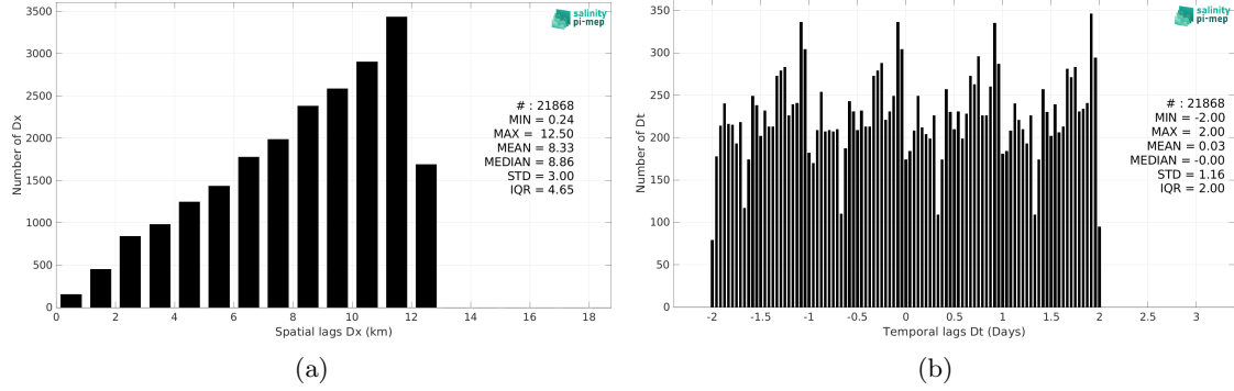
Figure 6: Histograms of the spatial (a) and temporal (b) lags between the location/time of the TSG (Polarstern) measurement and the date of the corresponding SMAP SSS L4 OI v3 - Daily (ESR) SSS pixel.
