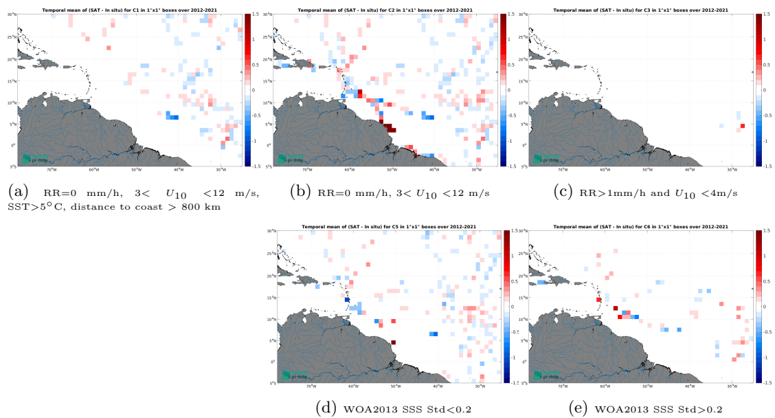
Figure 14: Temporal mean gridded over spatial boxes of size 1^\circ \times 1^\circ of \Delta SSS (SMAP SSS L4 OI v3 - Daily (ESR) - TSG (GOSUD-Sailing-ship)) for 5 different subdatasets corresponding to:RR=0 mm/h, 3 < U_{10} < 12 m/s, SST >5^\circ C, distance to coast > 800 km (a), RR=0 mm/h, 3 < U_{10} < 12 m/s (b), RR >1 mm/h and U_{10} < 4 m/s (c), WOA2013 SSS Std <0.2 (d), WOA2013 SSS Std >0.2 (e).
