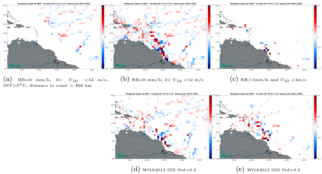
Figure 14: Temporal mean gridded over spatial boxes of size 1^\circ \times 1^\circ of \Delta\text{SSS} (SMAP SSS L4 OI v3 - Daily (ESR) - TSG (GOSUD-Research-vessel)) for 5 different subdatasets corresponding to: \text{RR}=0 \text{ mm/h}, 3 < U_{10} < 12 \text{ m/s}, \text{SST} > 5^\circ\text{C}, \text{distance to coast} > 800 \text{ km} (a), \text{RR}=0 \text{ mm/h}, 3 < U_{10} < 12 \text{ m/s} (b), \text{RR} > 1 \text{ mm/h and } U_{10} < 4 \text{ m/s} (c), \text{WOA2013 SSS Std} < 0.2 (d), \text{WOA2013 SSS Std} > 0.2 (e).
