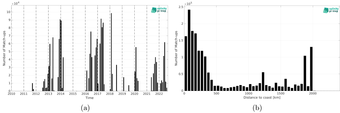
Figure 2: Number of match-ups between TSG (GOSUD-Research-vessel) and SMAP SSS L4 OI v3 - Daily (ESR) SSS as a function of time (a) and as function of the distance to coast (b) over the Amazon and Orinoco river plumes Pi-MEP region and for the full satellite product period.
